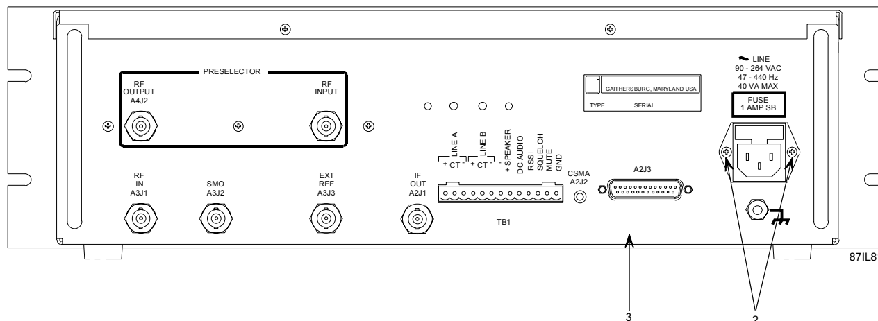
Figure 7-22. Filter/ Power (FL1J1) Removal and Replacement Procedures (Part 2)
