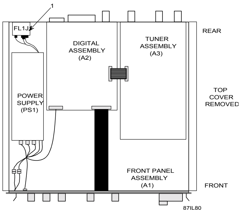
Figure 7-21. Filter/ Power (FL1J1) Removal and Replacement Procedures (Part 1)
