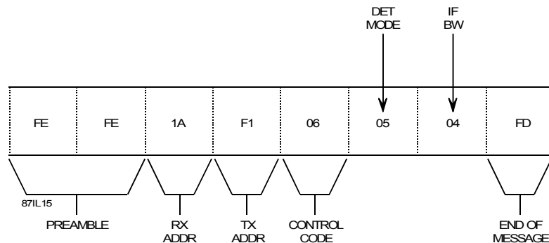
Figure 5-10. Detection Mode/ IF Bandwidth Command Format With Acknowledge
