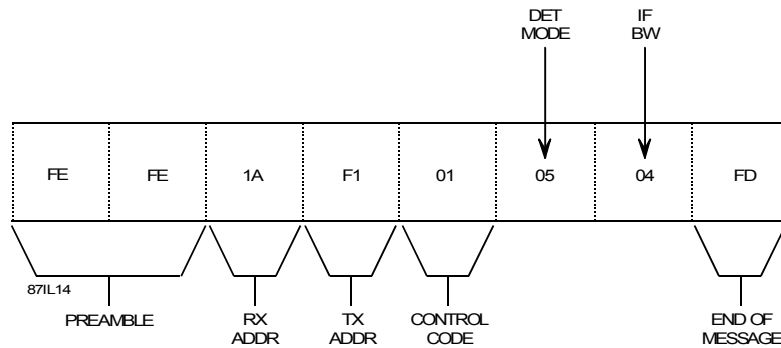
Figure 5-9. Detection Mode/ IF Bandwidth Command Format Without Acknowledge
