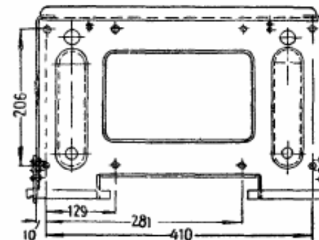
Receiver's mount
