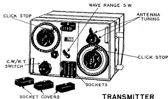
TRANSMITTER
