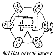
BOTTOM VIEW OF SOCKET
