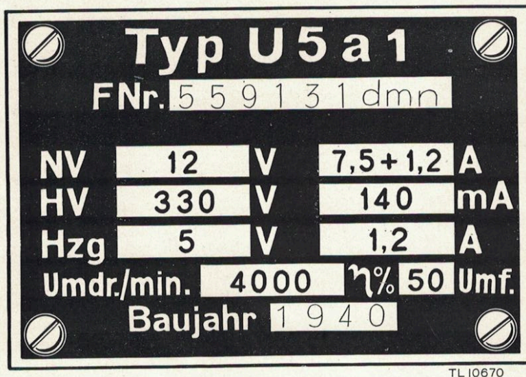
Figure 4. Nameplate of German dynamotor U5a1.
