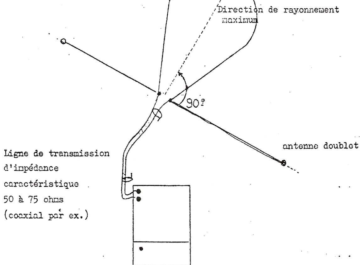
ANTENNE DOUBLET
