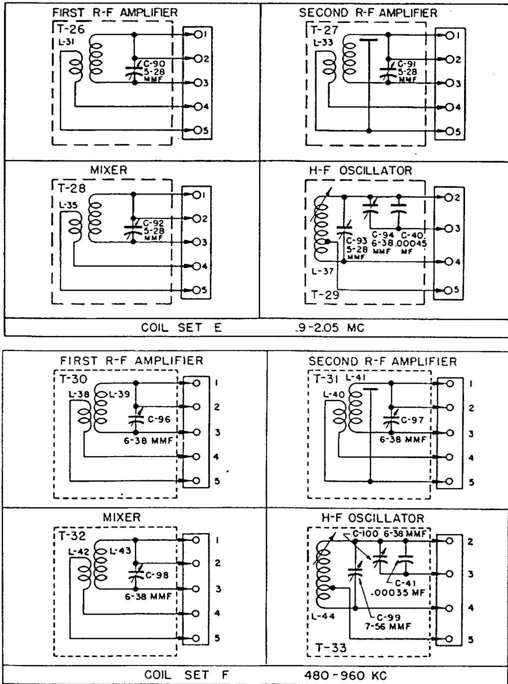
Figure 52. Coil sets E and F—schematic wiring diagram.
