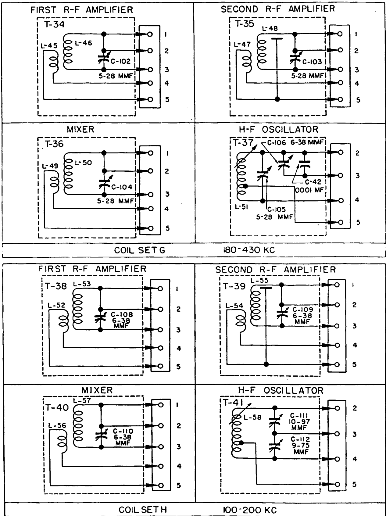
Figure 53. Coil sets G and H—schematic wiring diagram.
