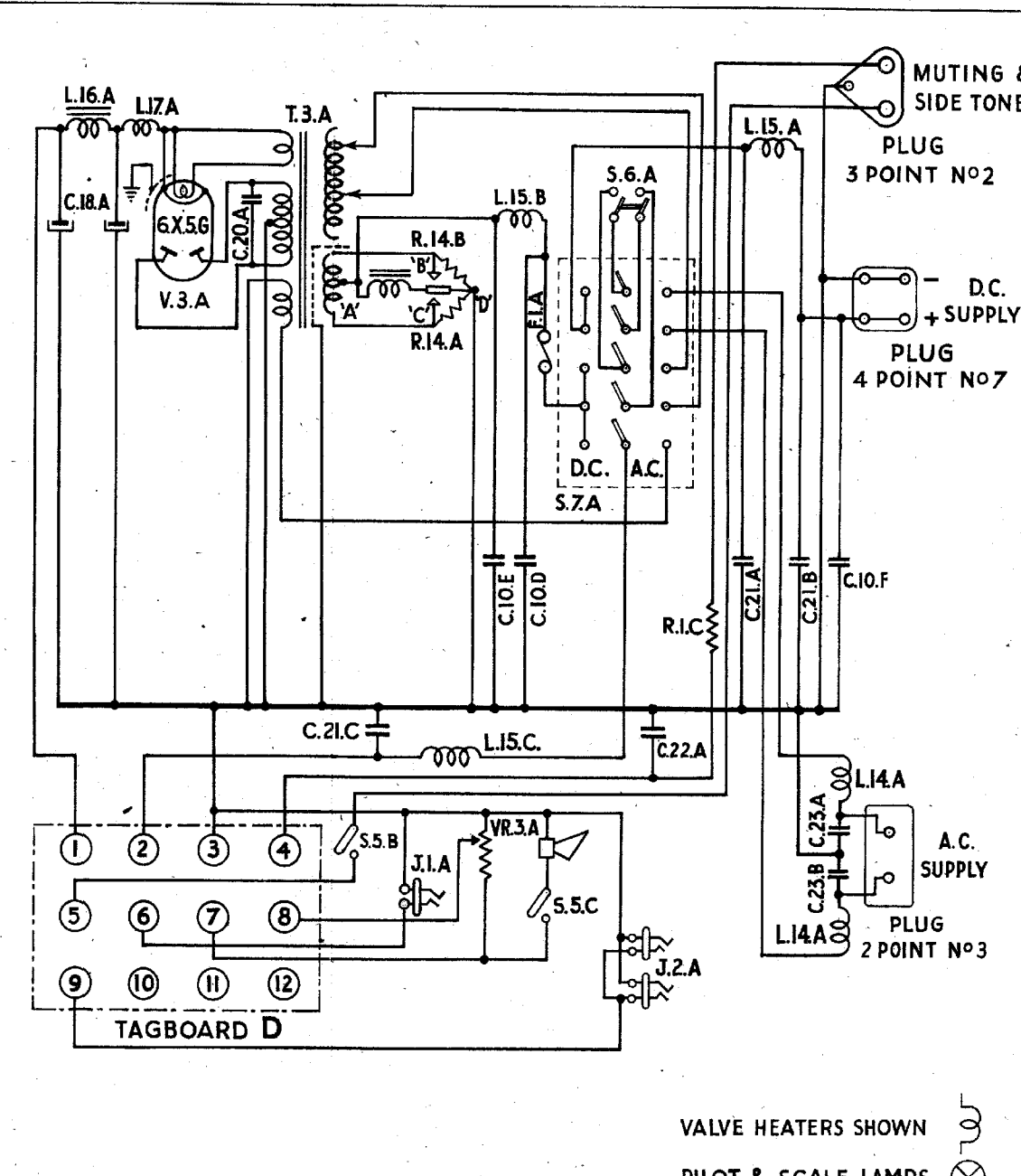
POWER UNIT
