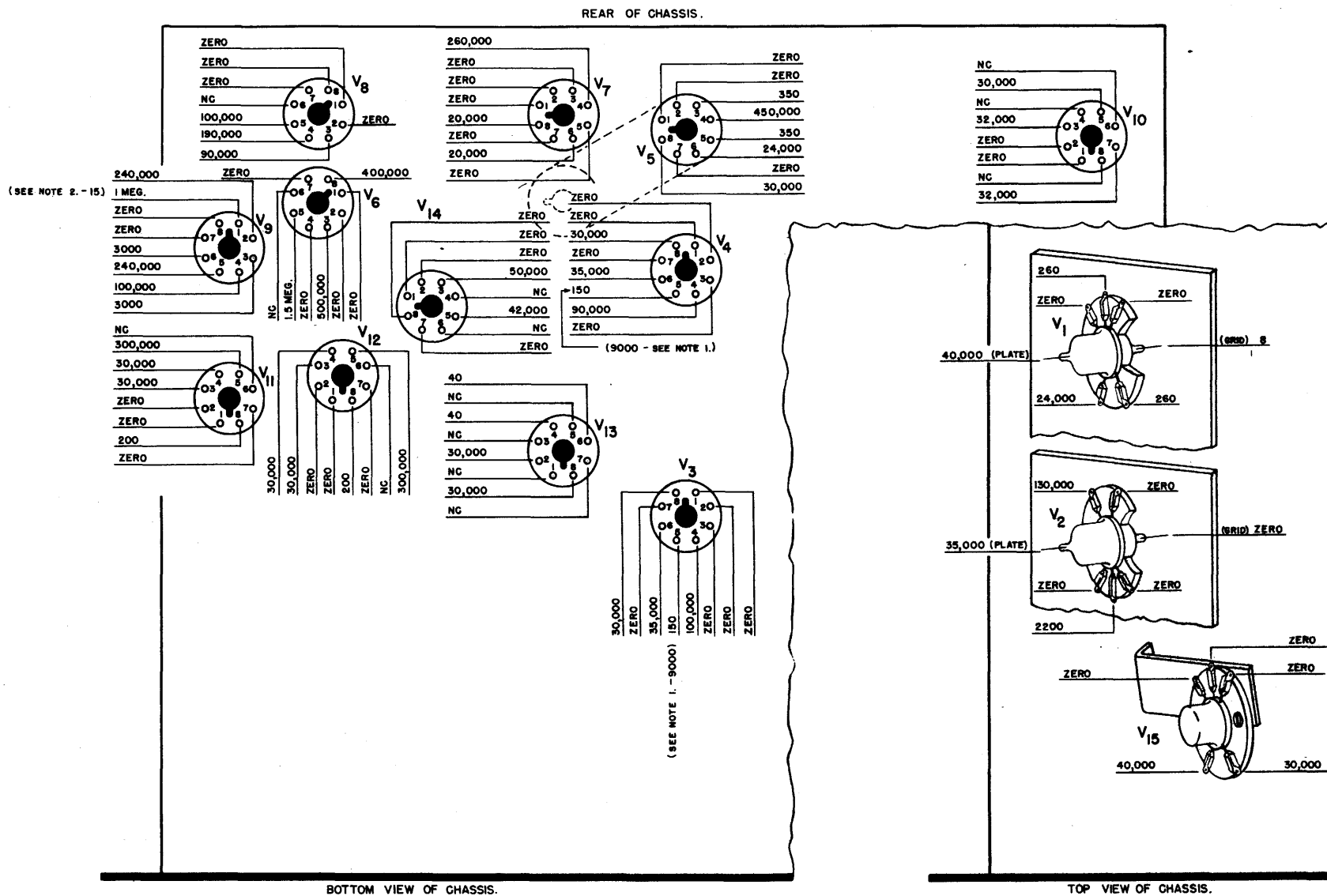
Figure 7-10: Radio Receiver Resistance Chart.
