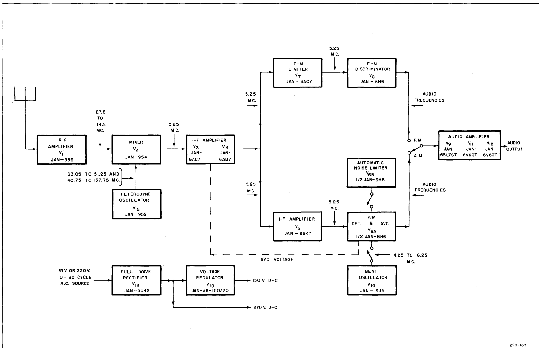
Figure 2-1: Types CHL-46130-C and CHL-46130-D Receiver Functional Block Diagram.
