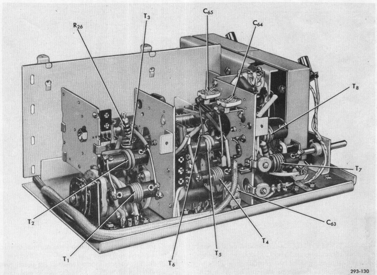
Figure 7-5: R-F Assembly, Rear Oblique View.
