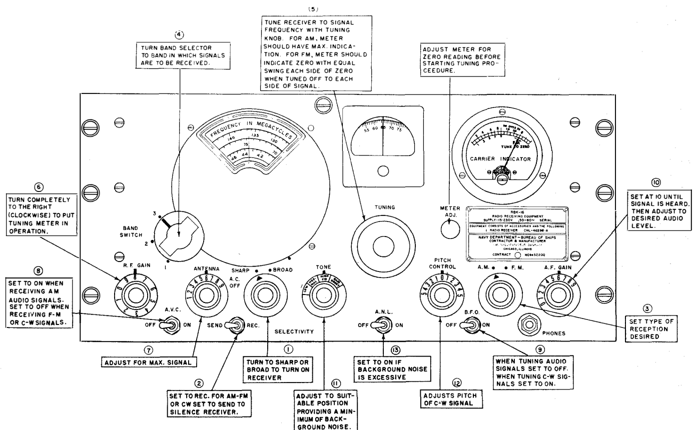
Figure 4-2. Radio Receiving Equipment Navy Model RBK-16, Tuning Adjustments.
