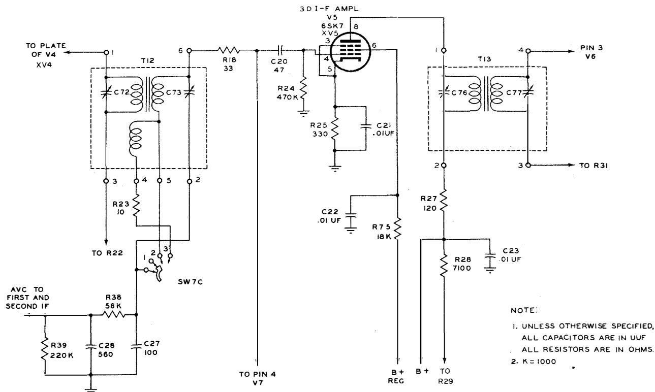
Figure 2-6. Radio Receiving Equipment Navy Model RBK-16, I-f Amplifier, Simplified Schematic Diagram.
