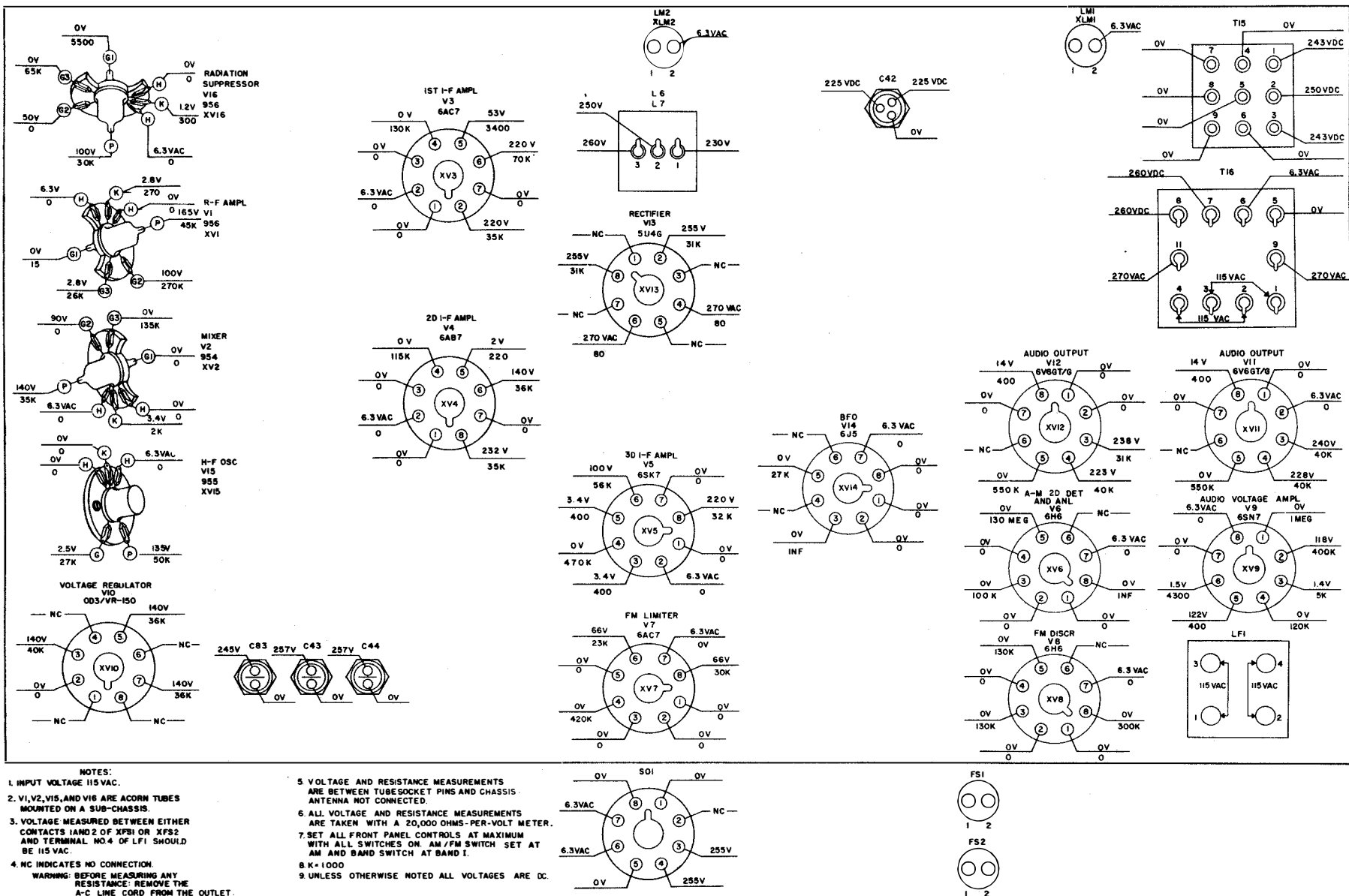
Figure 7-3. Radio Receiving Equipment Navy Model RBK-16, Voltage and Resistances at Tube Sockets.
