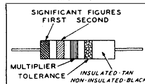
AXIAL TYPE
