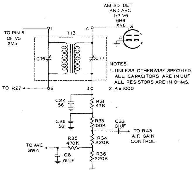
Figure 2-8. Radio Receiving Equipment Navy Model RBK-16, A-m 2d Detector and Avc, Simplified Schematic Diagram.
