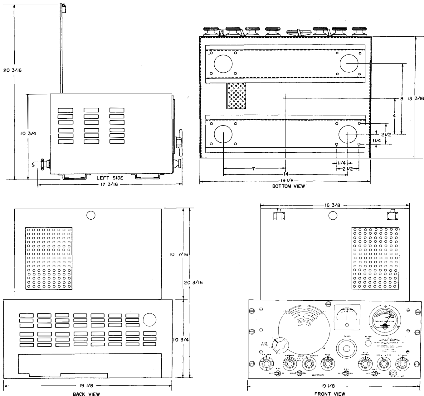
Figure 3-2. Radio Receiving Equipment Navy Model RBK-16, Dimensional Drawing Having Three Views.
