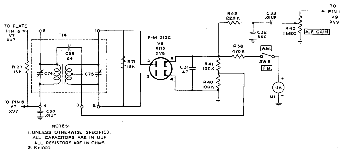
Figure 2-11. Radio Receiving Equipment Navy Model RBK-16, F-m Discriminator, Simplified Schematic Diagram.
