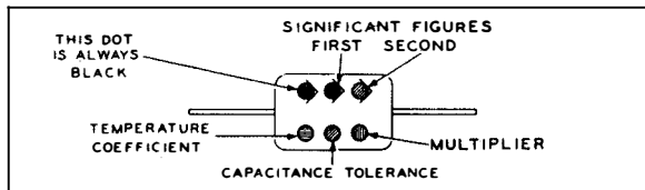
JAN 6-DOT COLOR CODE FOR MICA-DIELECTRIC CAPACITORS
