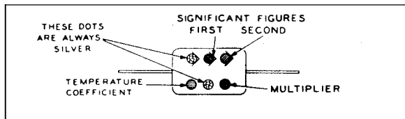
JAN 6-DOT COLOR CODE FOR PAPER-DIELECTRIC CAPACITORS
