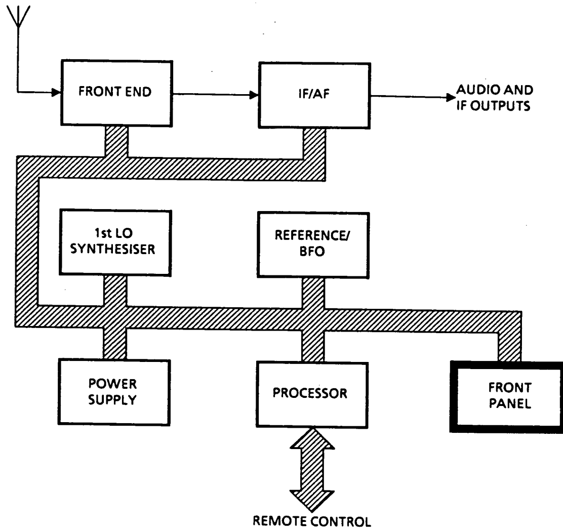
Fig. 16.1 Receiver Block Diagram
