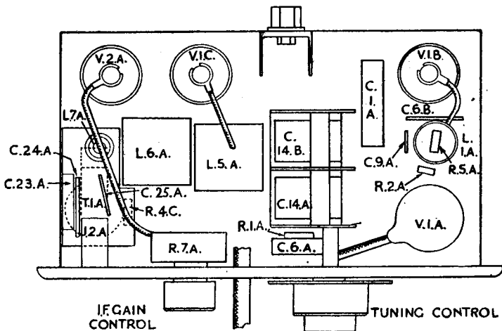
FIG. 9. TOP VIEW OF CHASSIS
