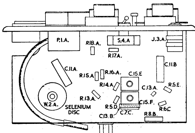
FIG. 12. UNDERSIDE VIEW OF CHASSIS
