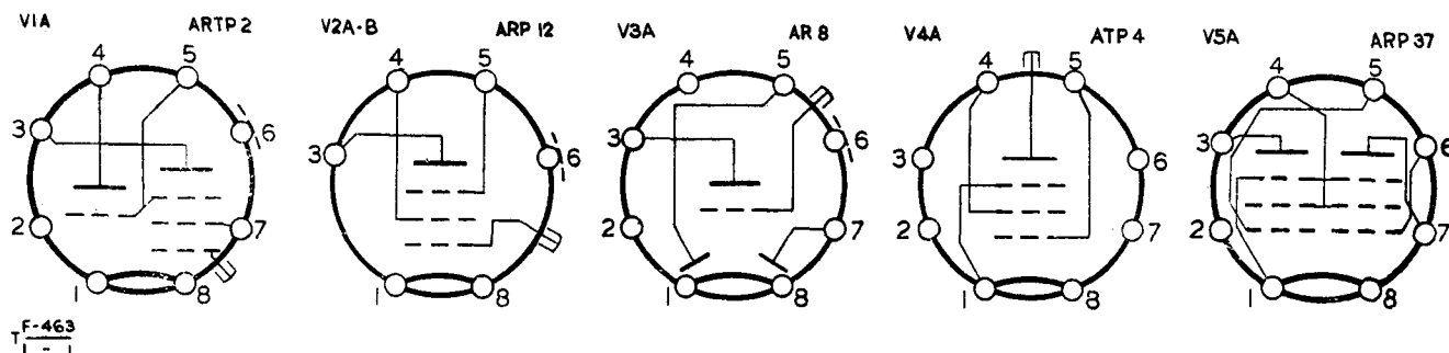
Fig. 1—Valve bases
