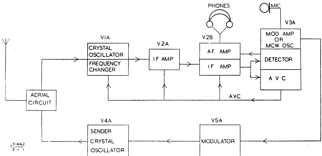
Fig. 1—Block diagram
