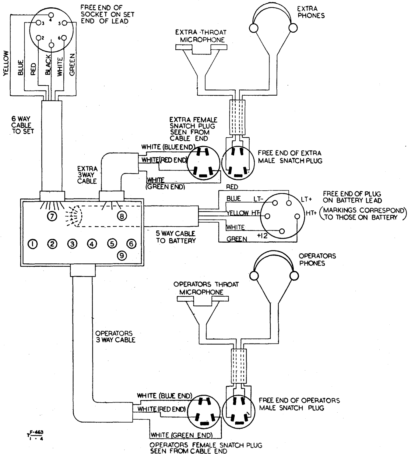
Fig. 4—External connections to set
