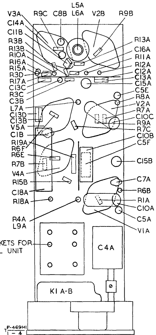
Fig. 4—Component layout, bottom
