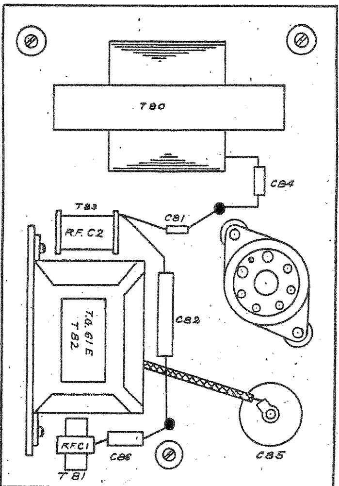
TOP VIEW
