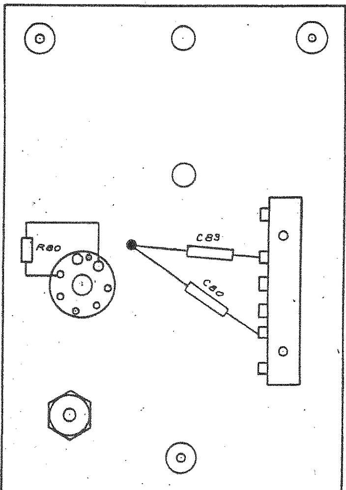
UNDERSIDE VIEW
