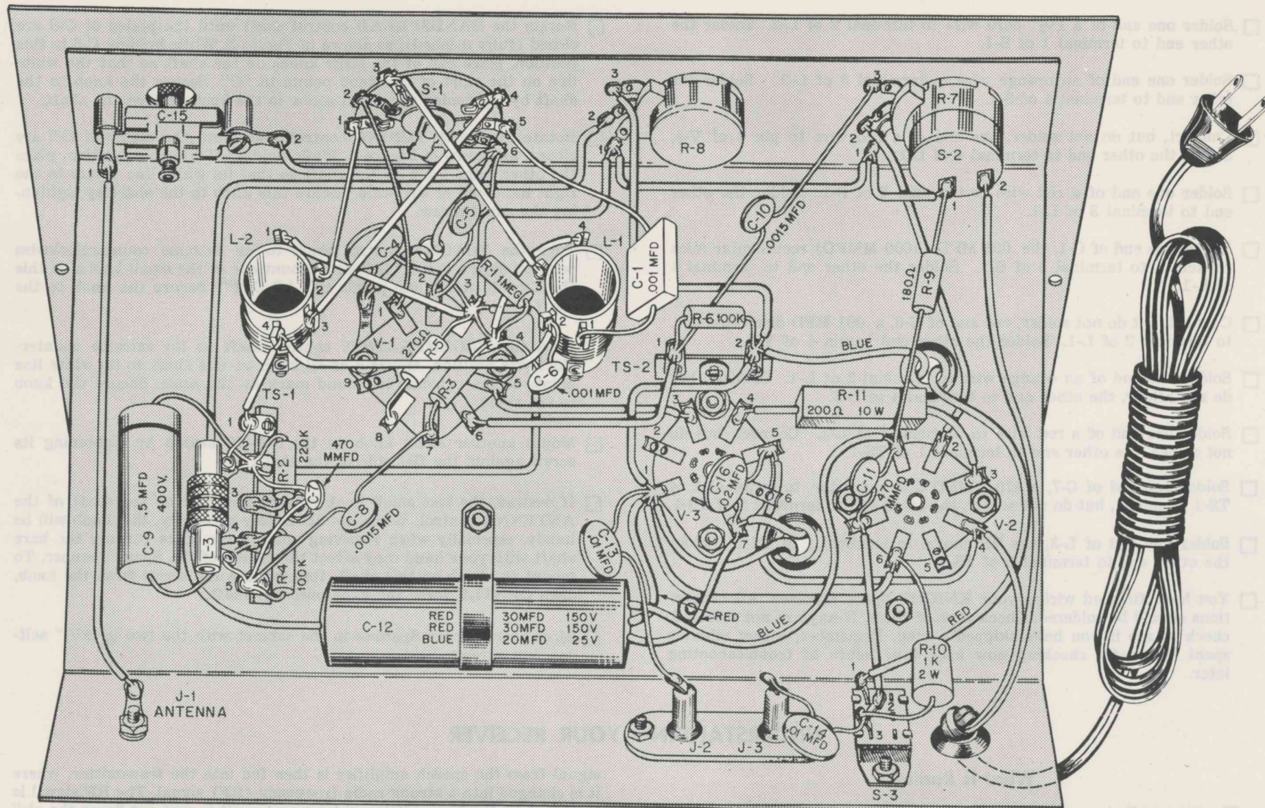
FIGURE 8. SECOND CHASSIS WIRING VIEW
