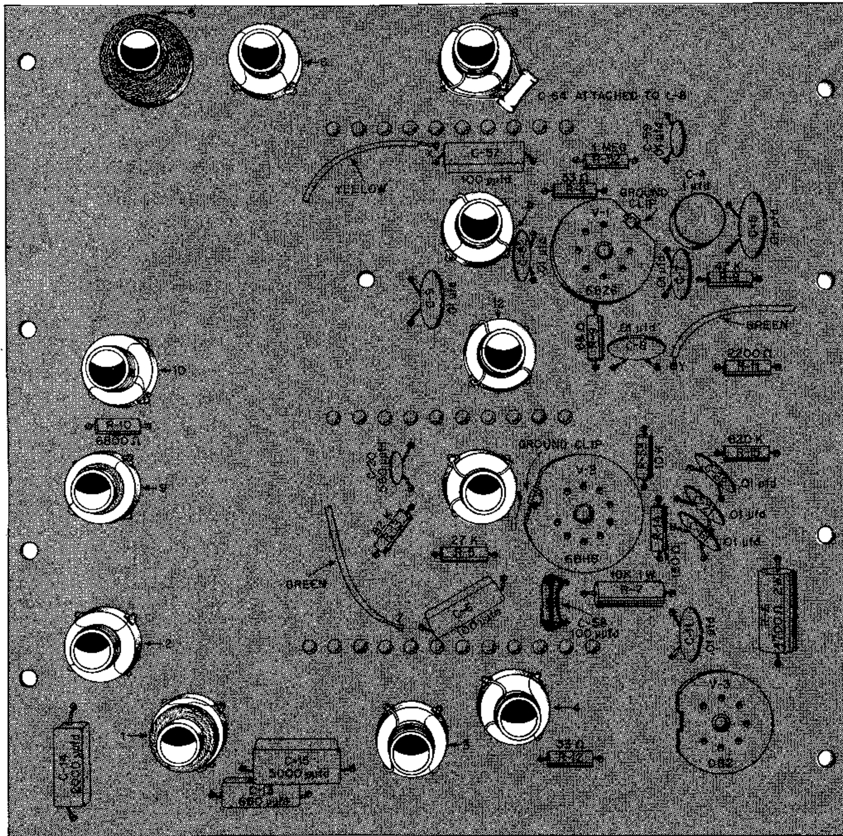
FIGURE 13. MOUNTING THE COILS
