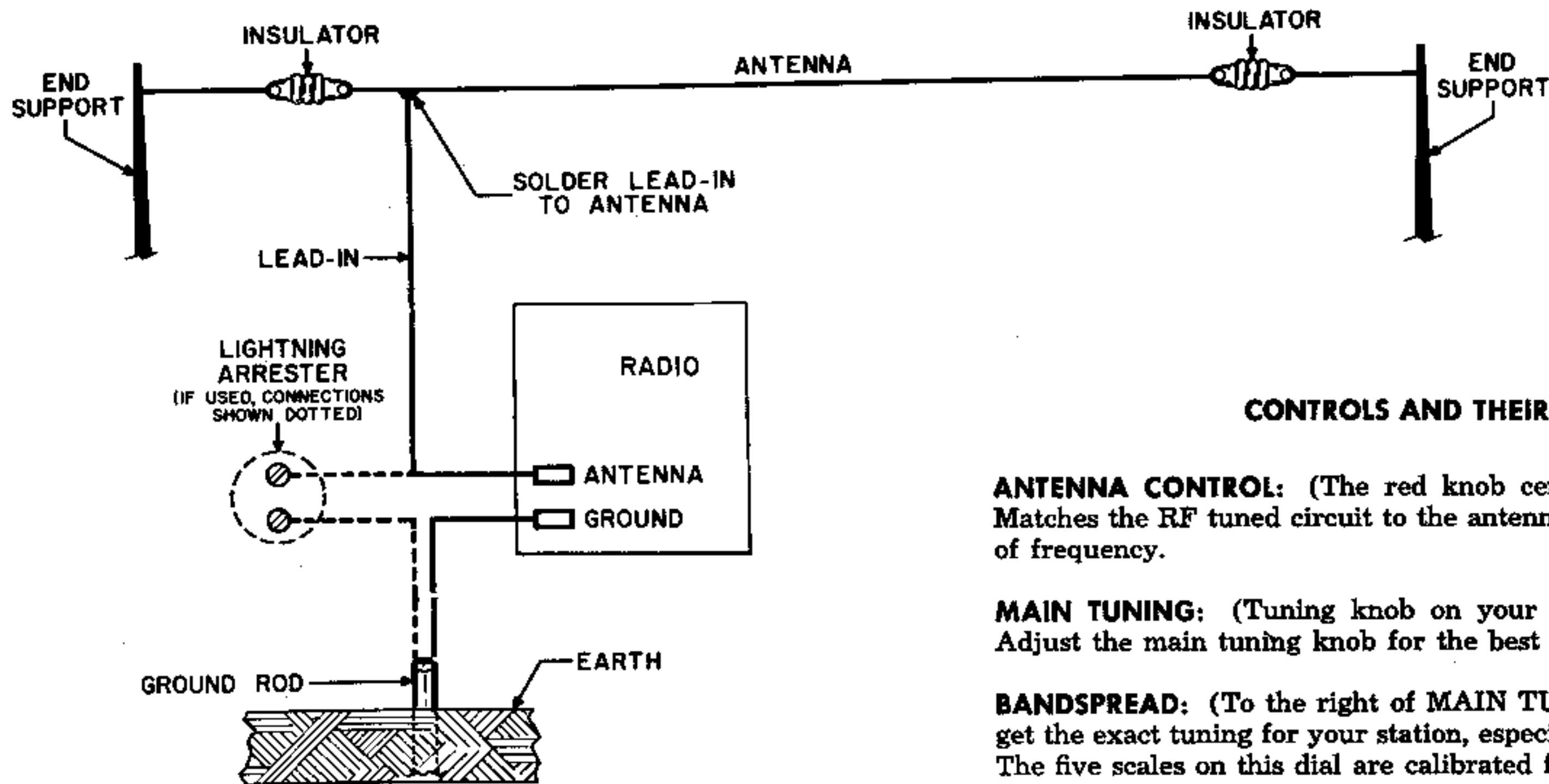
FIGURE 25. INSTALLING AN ANTENNA
