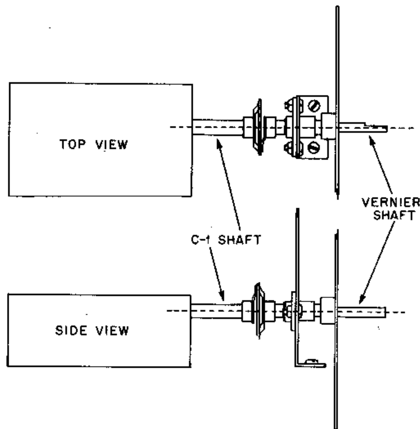
FIGURE 20A. SHAFT ALIGNMENT
