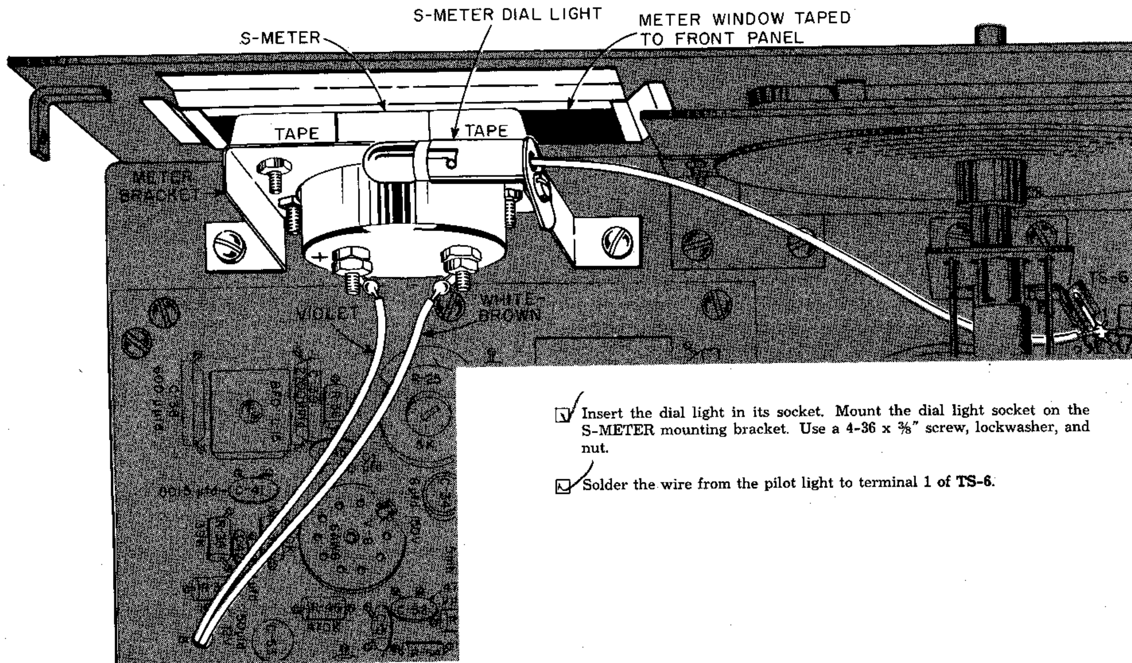
FIGURE 27. INSTALLING THE S-METER
