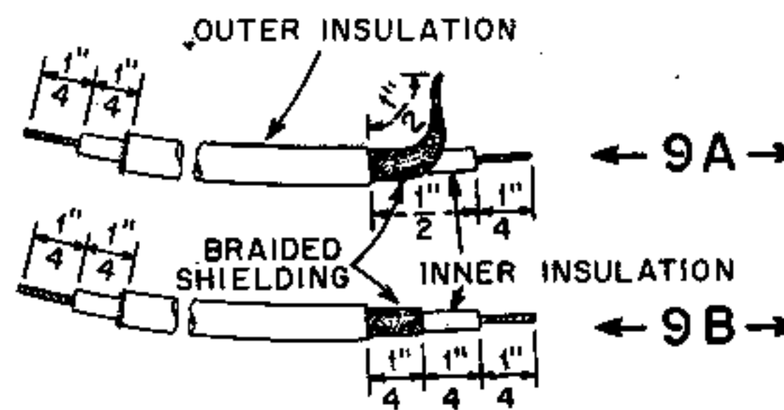
FIGURE 9. PREPARING INSULATED SHIELDED WIRES
