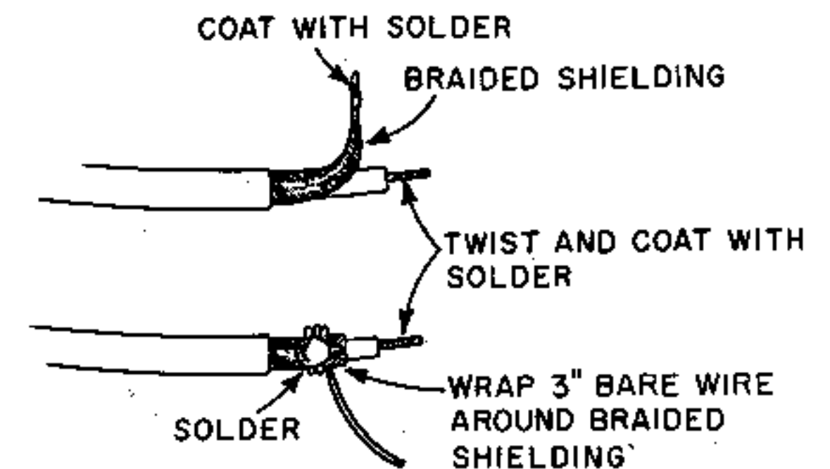
FIGURE 9. PREPARING INSULATED SHIELDED WIRES
