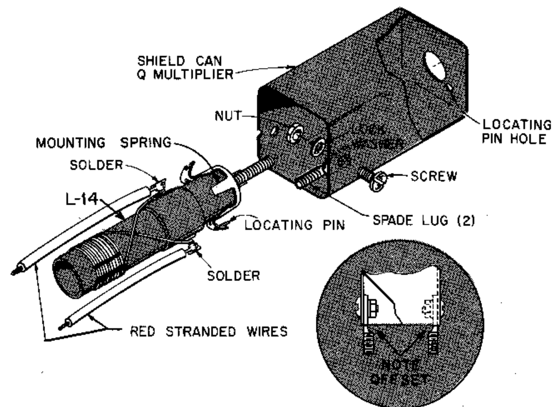
FIGURE 2. MOUNTING THE QX COIL
