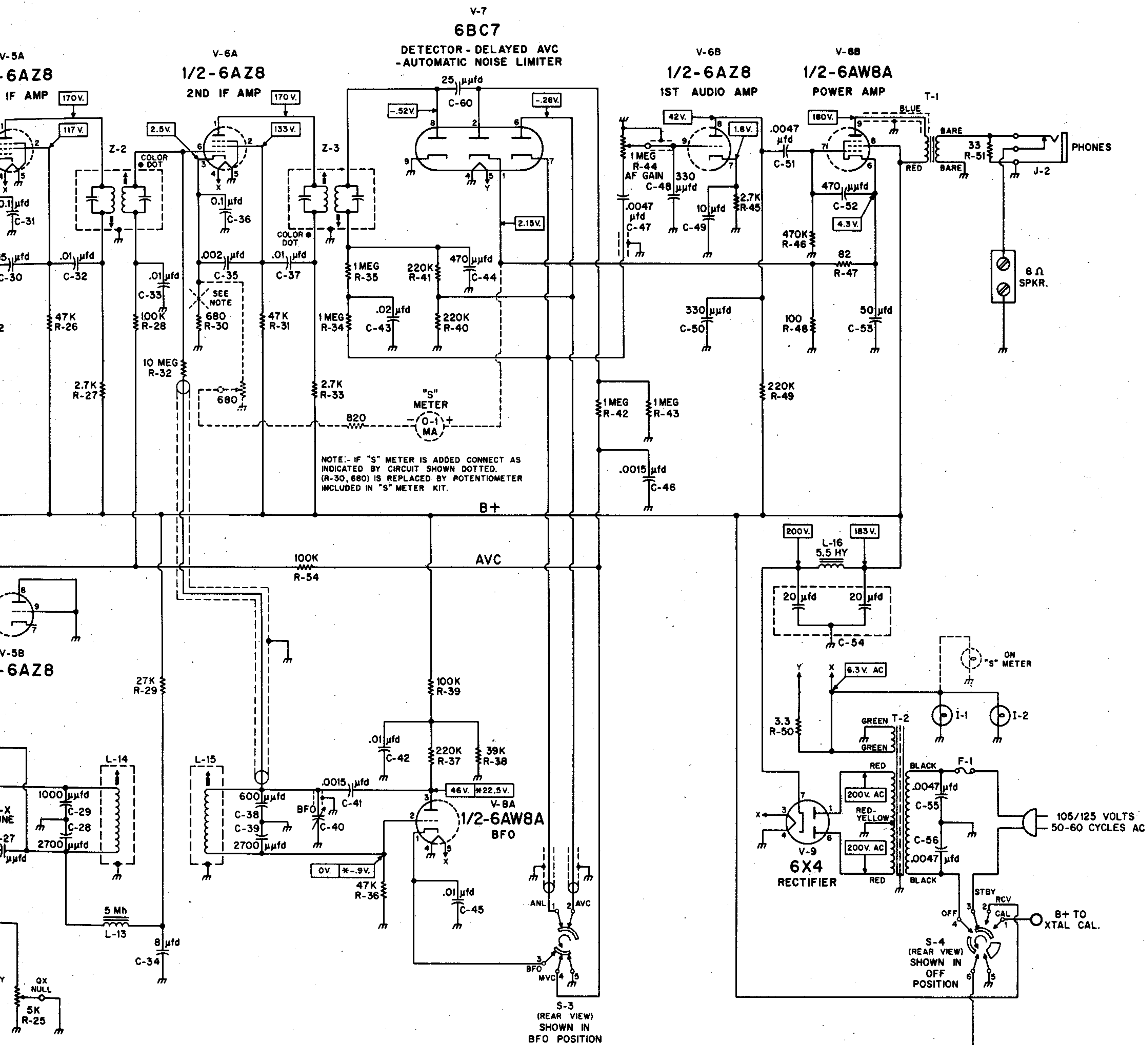
FIGURE 29 SCHEMATIC DIAGRAM
