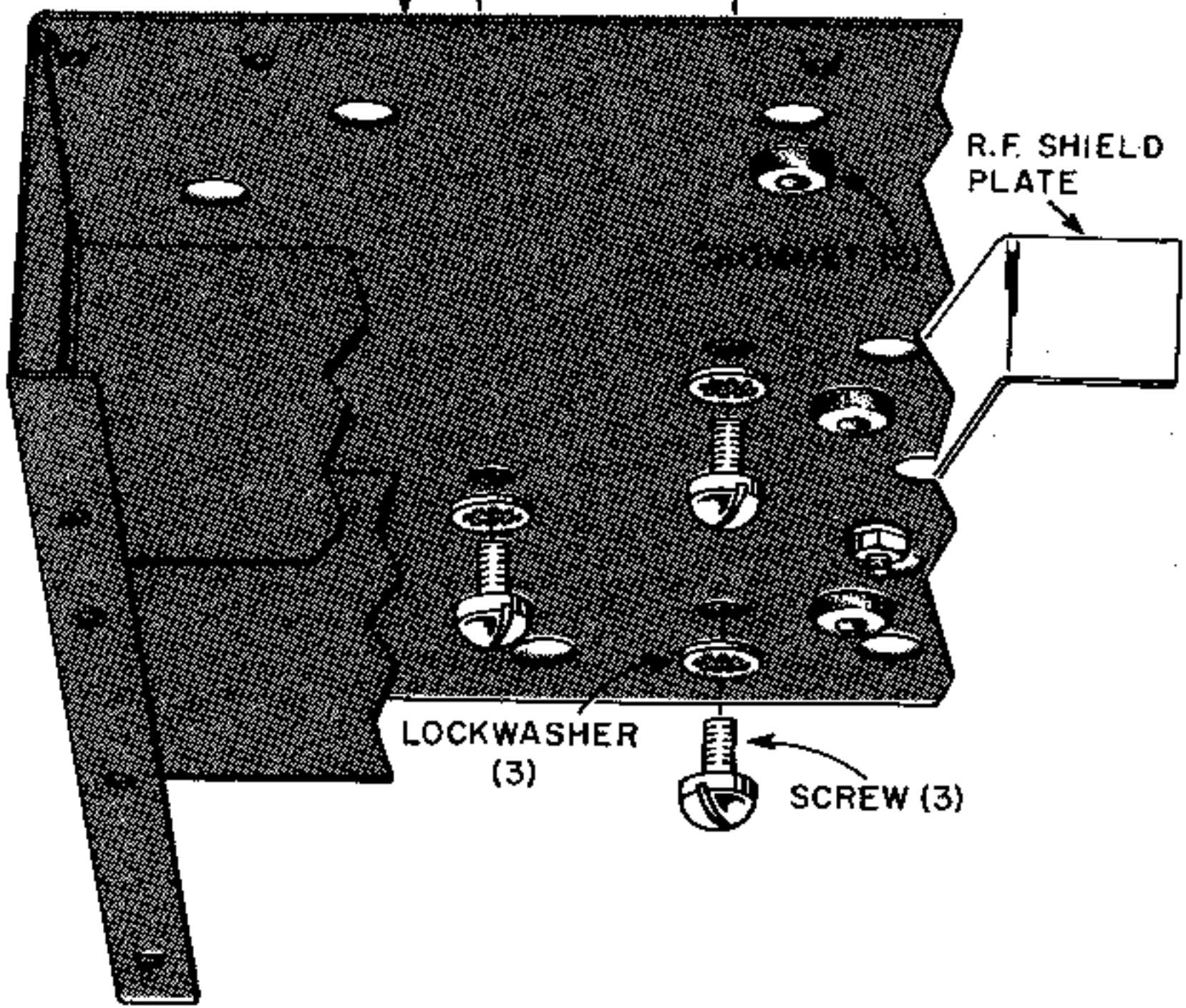
FIGURE 17. MOUNTING C-1 (MAIN TUNING CAPACITOR)
