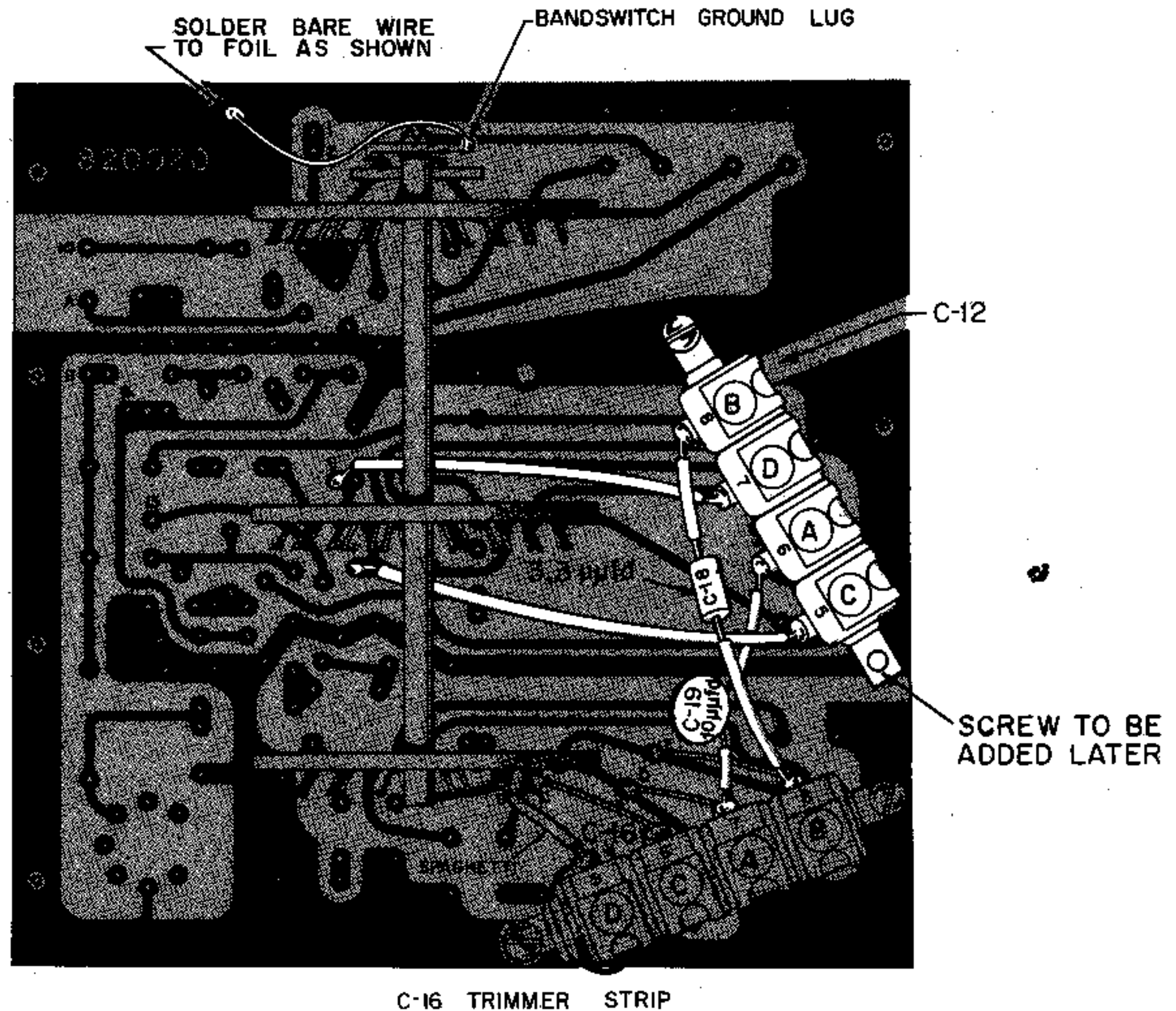
FIGURE 16. MOUNTING C-12 (TRIMMER STRIP)
