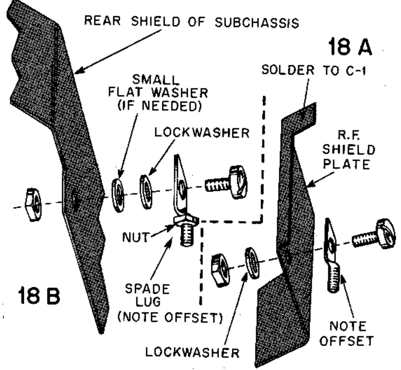
FIGURE 18. MOUNTING THE SPADE LUGS
