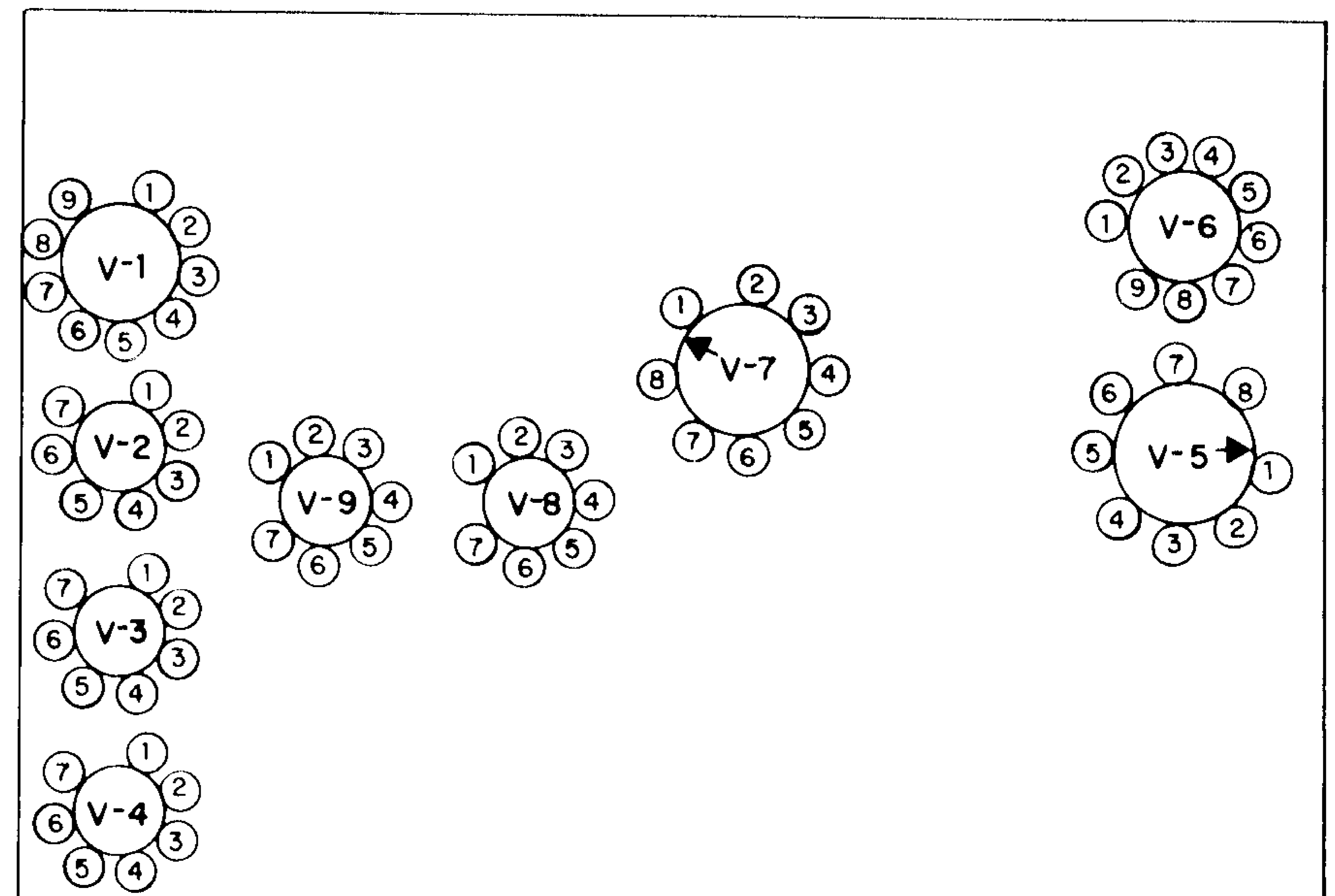
TUBE LOCATION (bottom view)
