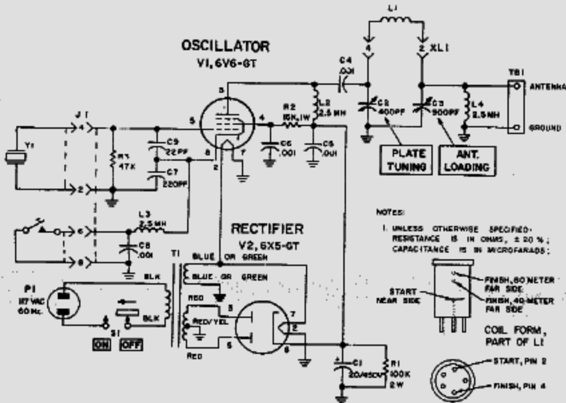
AC-1 SCHEMATIC DIAGRAM
