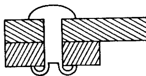
PROPERLY ROLLED SEMITUBULAR RIVET
