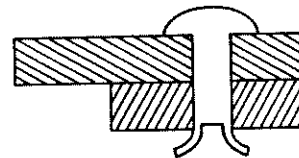
IMPROPERLY ROLLED SEMITUBULAR RIVET
