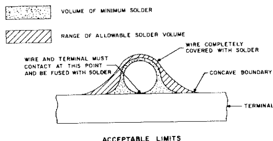
Figure 1-20. Section Showing Acceptable Limits of Solder Volume
