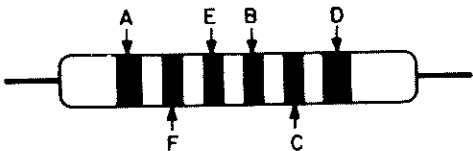
Tubular Capacitors (Old RMA)
