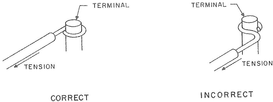
Figure 1-13. Avoiding Tension on Soldered Joint
