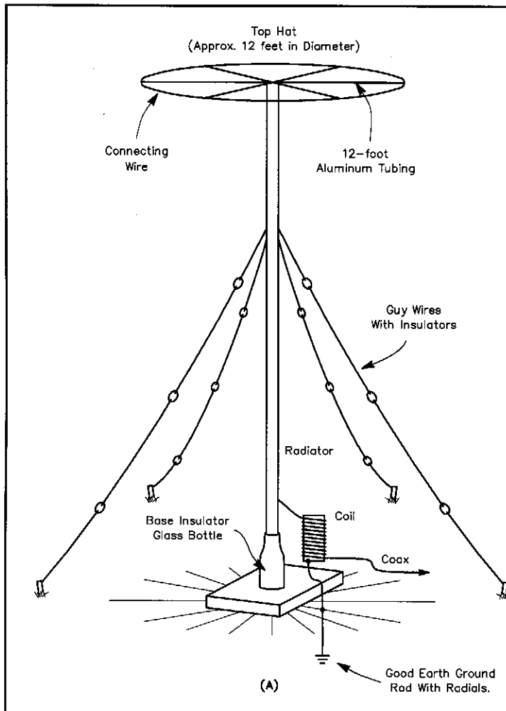
Figure 3—A typical 1750-meter transmitting antenna system (A). The radiator is topped with a "capacitance hat" and secured with several guy wires. A glass bottle insulates the base. The loading coil (B) connects between the radiator and the ground system with the feed line attached to the coil taps. The length of the radiator and feed line must conform to FCC Part 15 Rules. ("The total length of the transmission line, antenna and ground lead, if used, shall not exceed 15 meters.")
