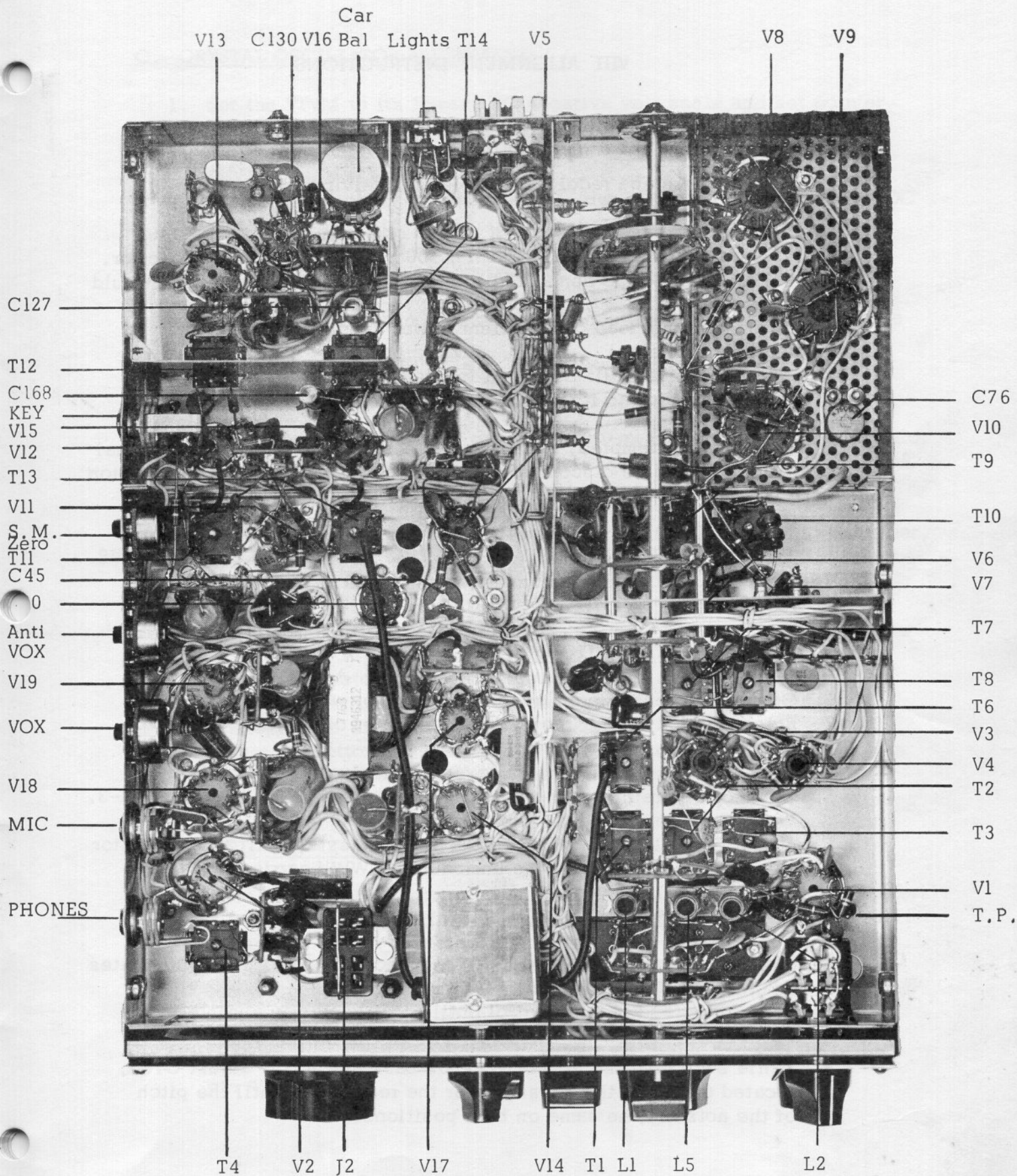
Figure 11 BOTTOM VIEW
