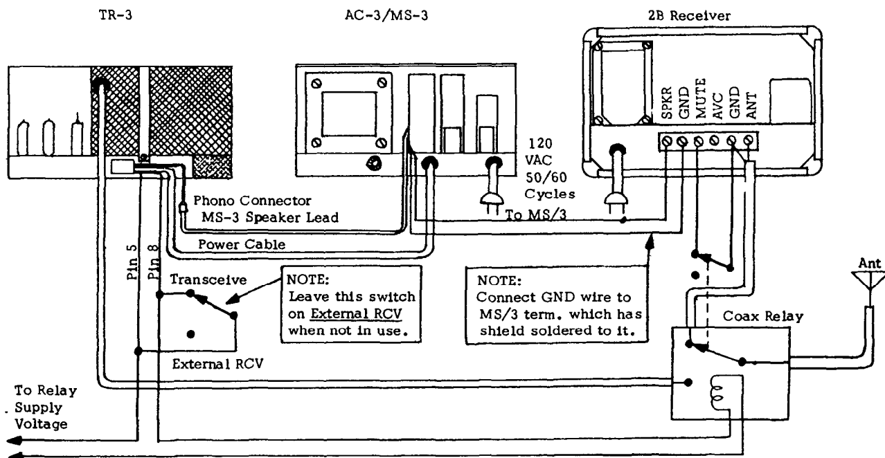
FIG. 3 USING THE TR-3 WITH AN EXTERNAL RECEIVER
