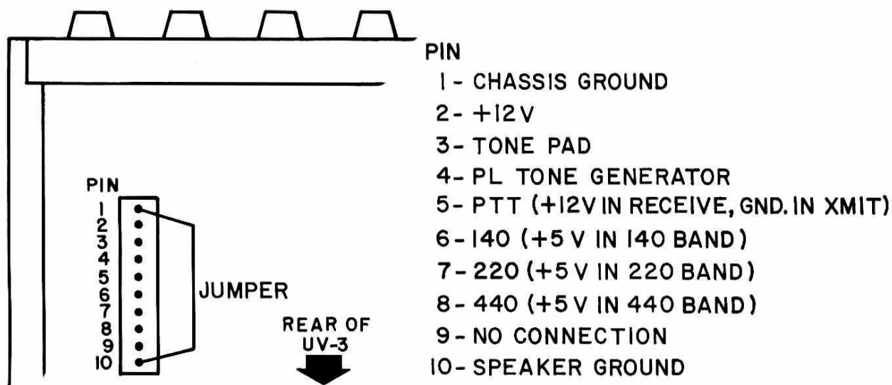
Figure 3-5. Auxiliary Connector
