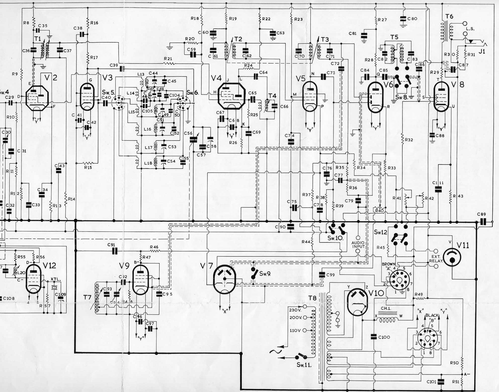
FLYSTONE "600" COMPONENT VALUES
