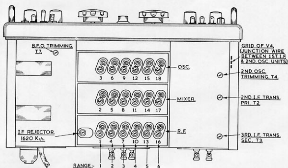
Fig. 4. Underside view of "888" Receiver in outline.
