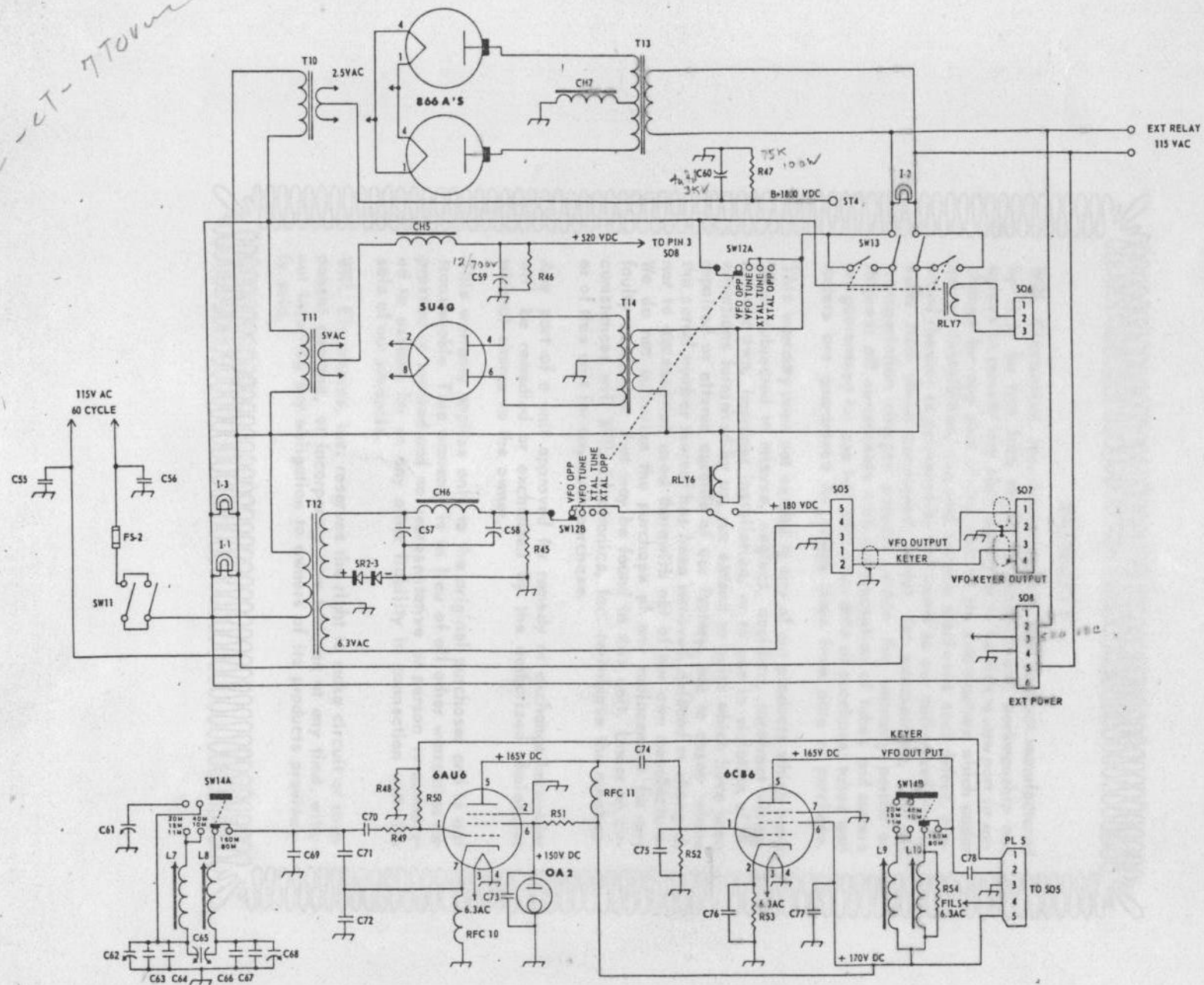
WRL 500C POWER SUPPLY AND VFO
