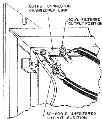
Fig. 4. Output Connector Changeover Link
