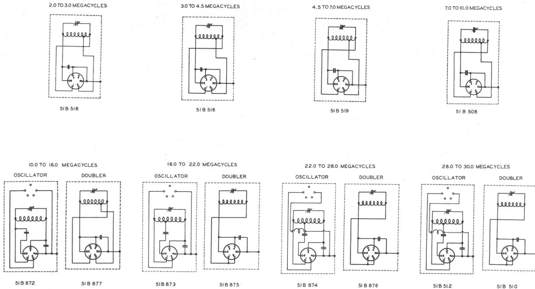
Figure 5. Tuning units for Model HT-9 Transmitter, schematic wiring diagrams.
