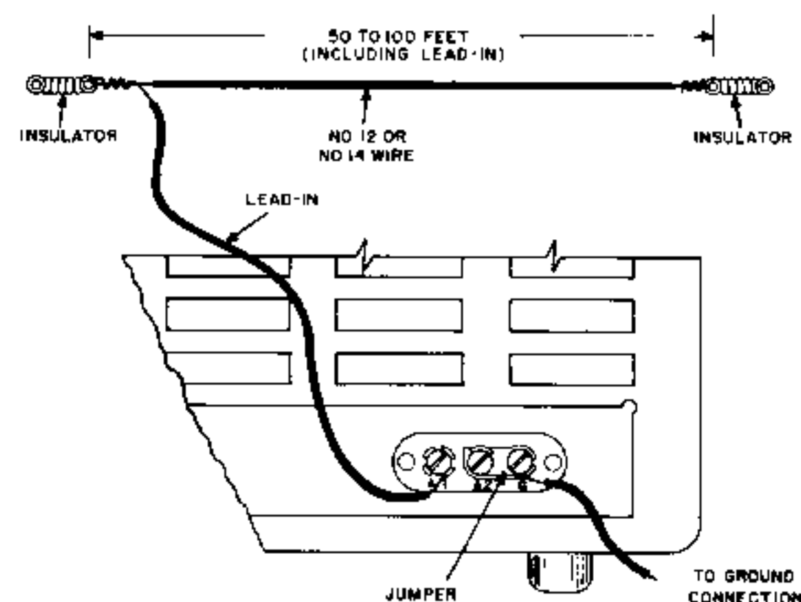
Fig. 3. Single Wire Antenna Installation 9281550
