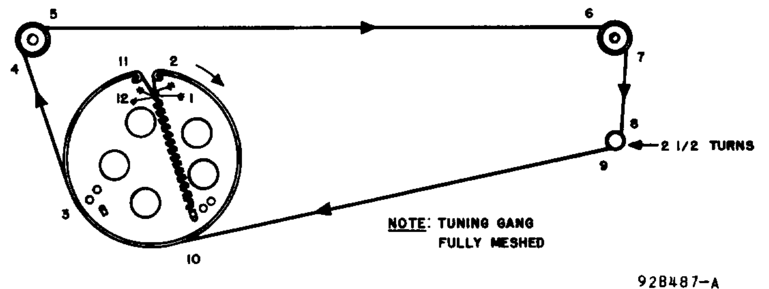
Fig. 7. TUNING Dial Cord Stringing Diagram
