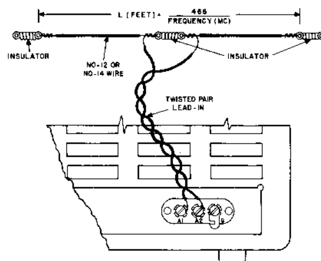
Fig. 4. Doublet Antenna Installation Using Twisted Pair Lead-In
