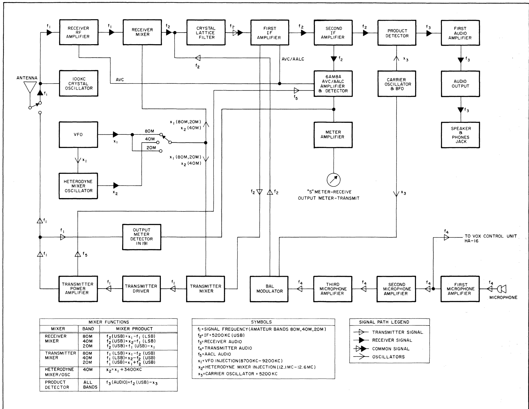
Figure 9. Block Diagram of Transceiver.
