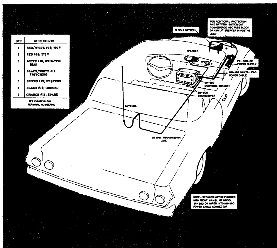
Figure 6. Wiring Diagram of Mobile Installation.
