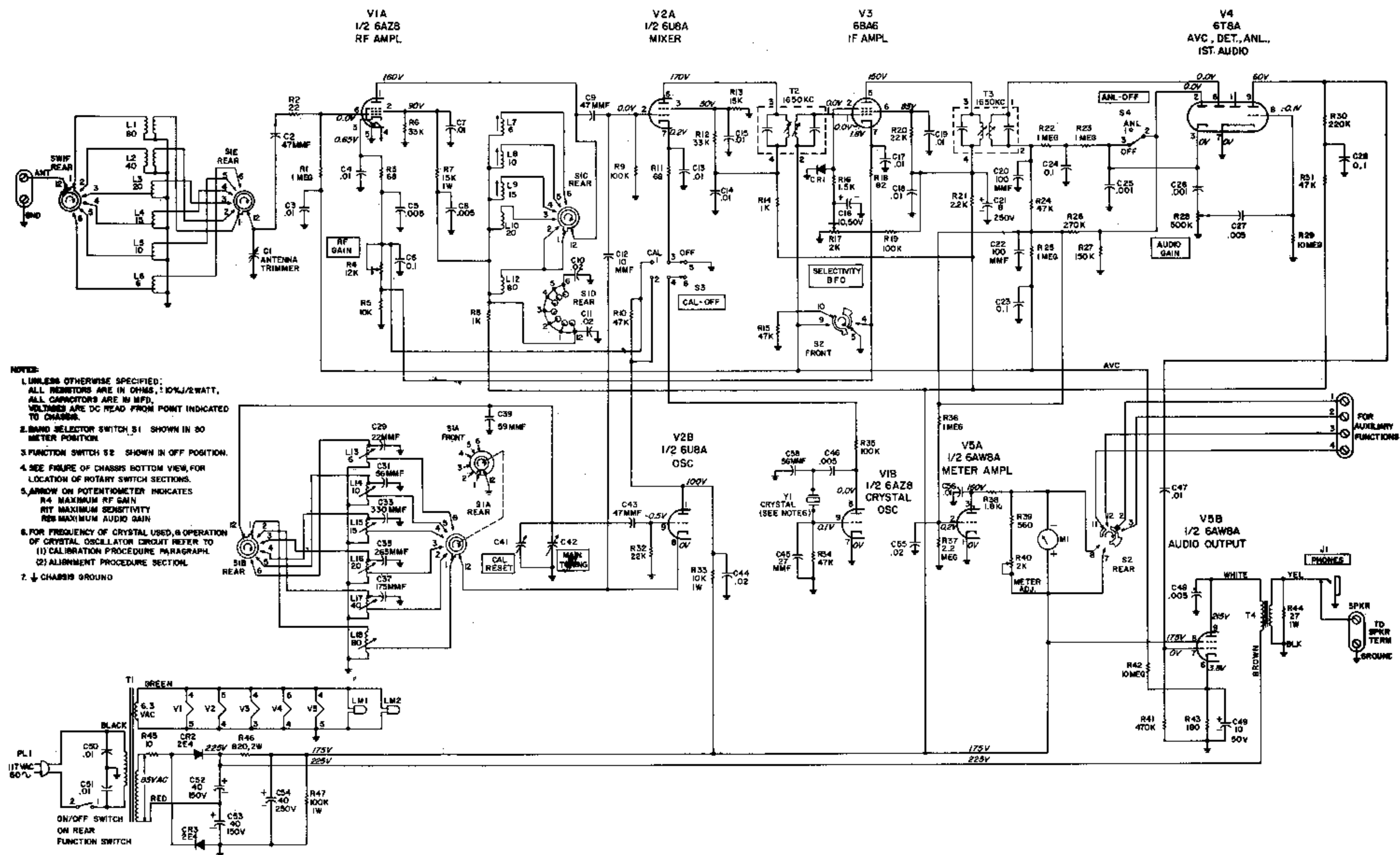
Figure 12. Schematic Drawing.
