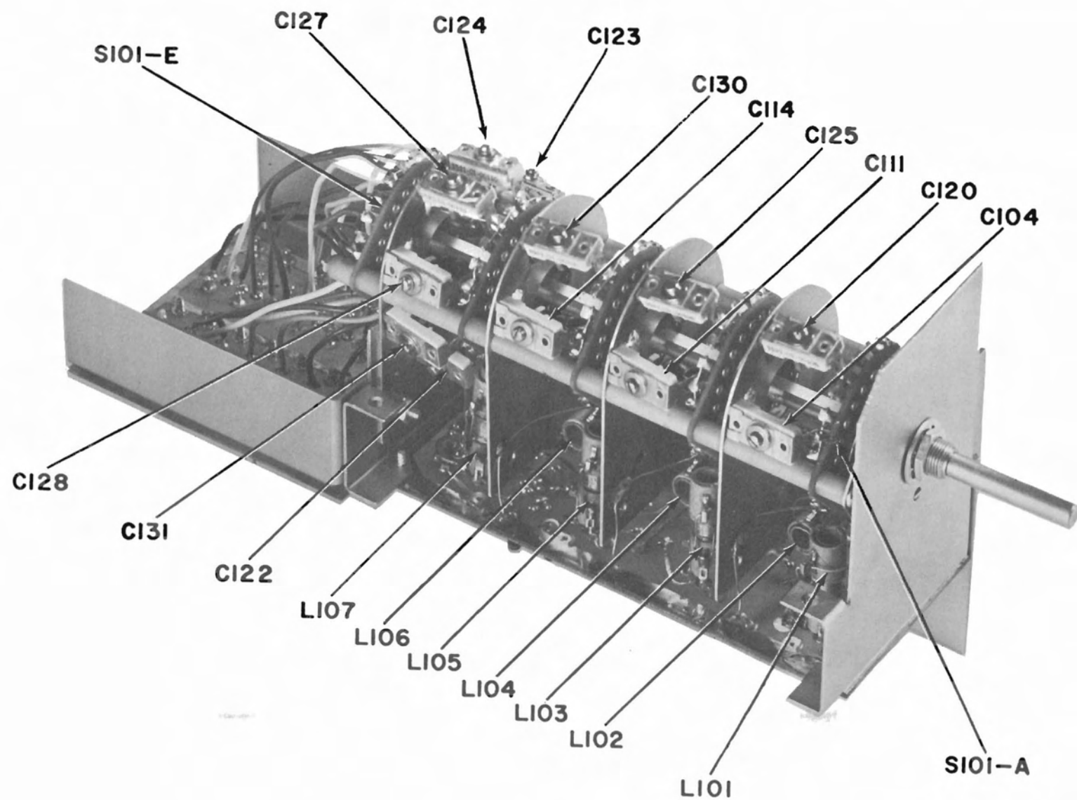
FIGURE 4-3 RF MODULE WITH BANDSWITCH
