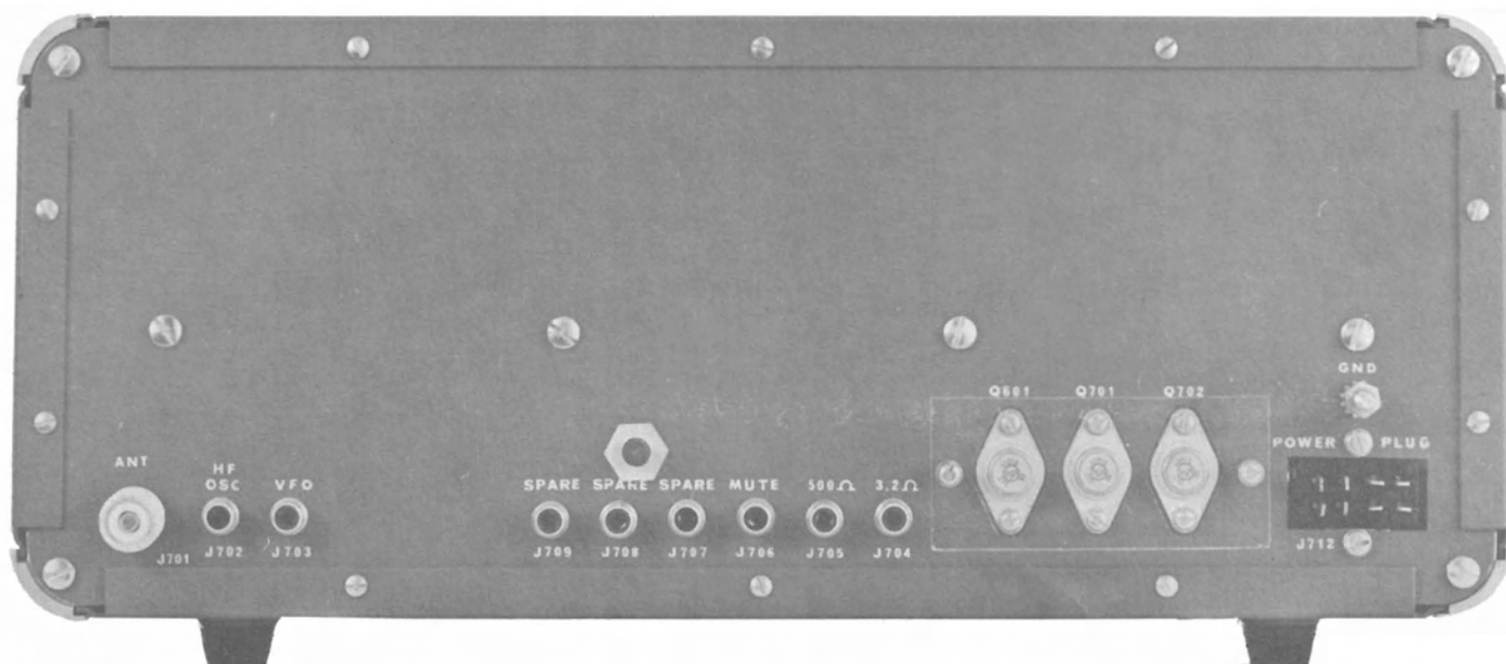
FIGURE I-1 REAR CONNECTIONS
