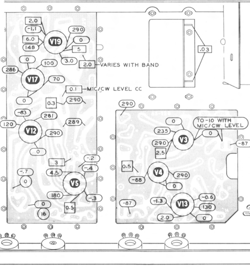
TRANSMITTER VOLTAGE CHART FIGURE 1-19
