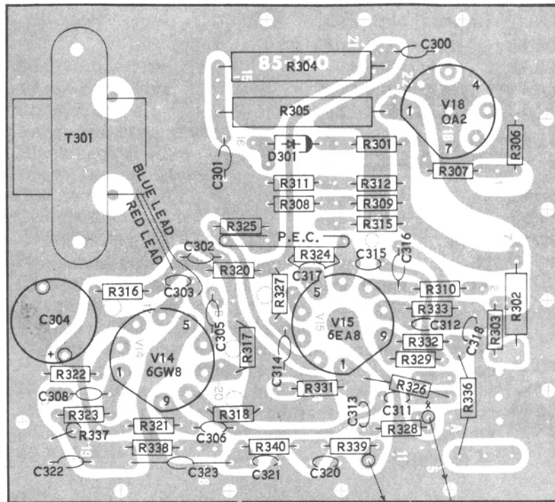
AUDIO CIRCUIT BOARD
