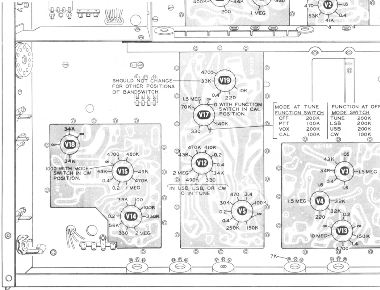
RESISTANCE CHART FIGURE 1-20
