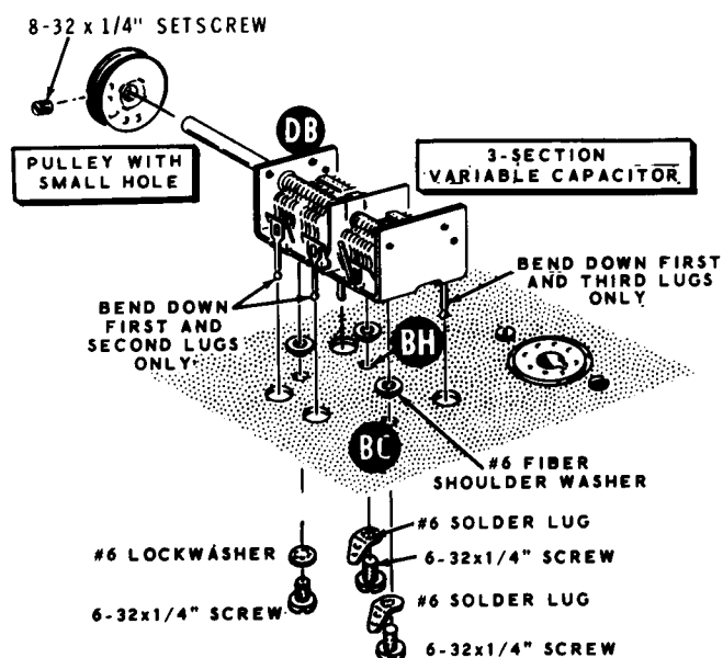
Detail 8-3A
