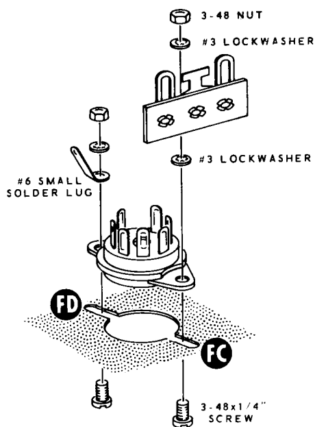
Detail 7-1A
