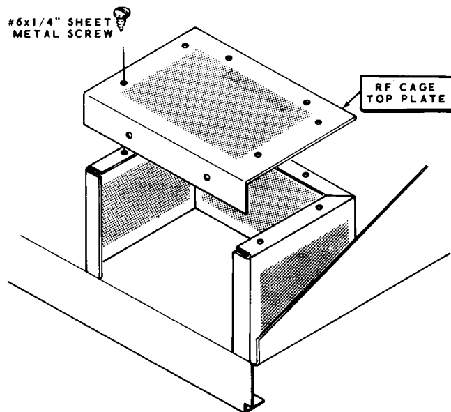
Detail 8-8D
