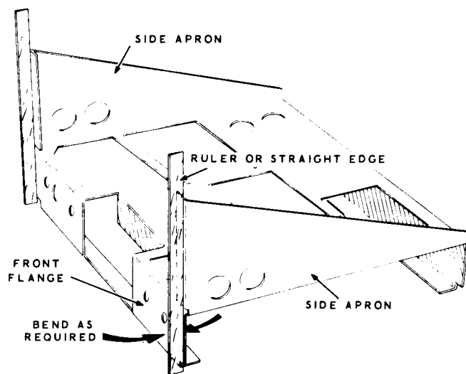
Detail 8-1A
