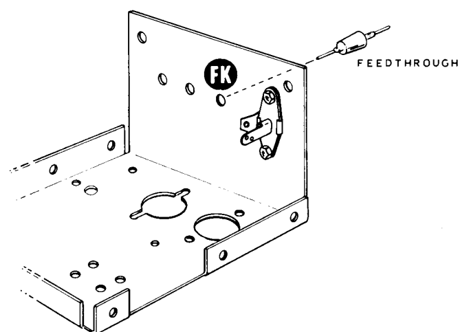
Detail 7-2C
