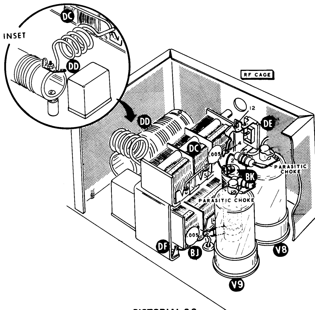
PICTORIAL 8-8 (Repeat)
