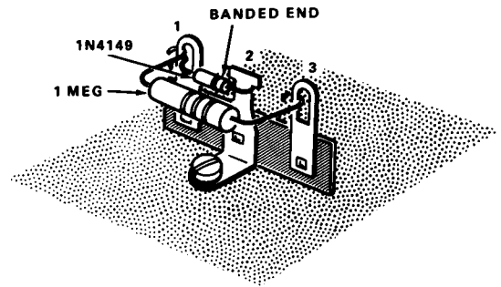
Detail 8-19C
