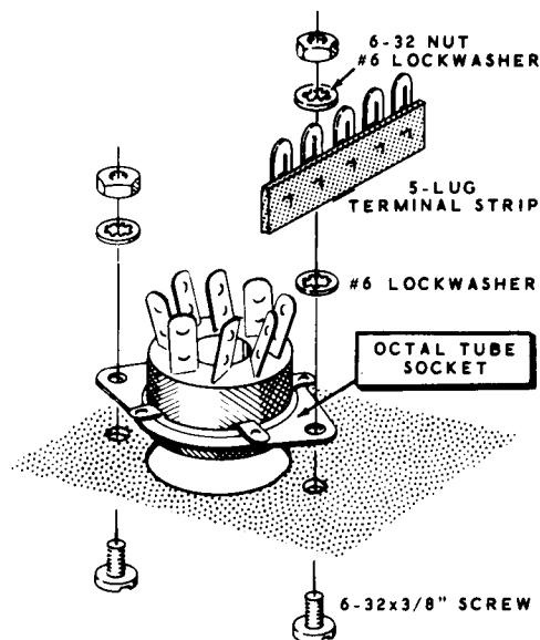
Detail 8-1G
