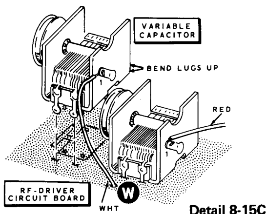
Detail 8-15C
