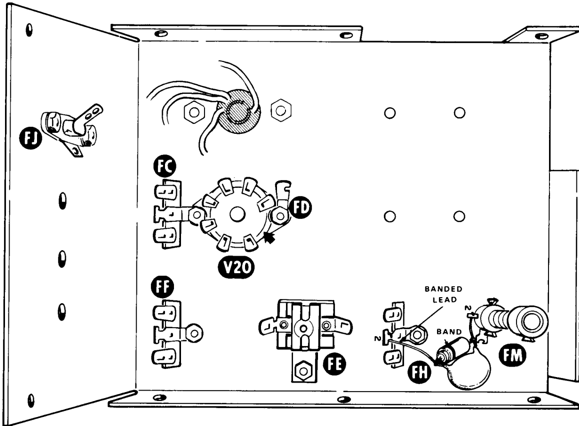
PICTORIAL 7-3
