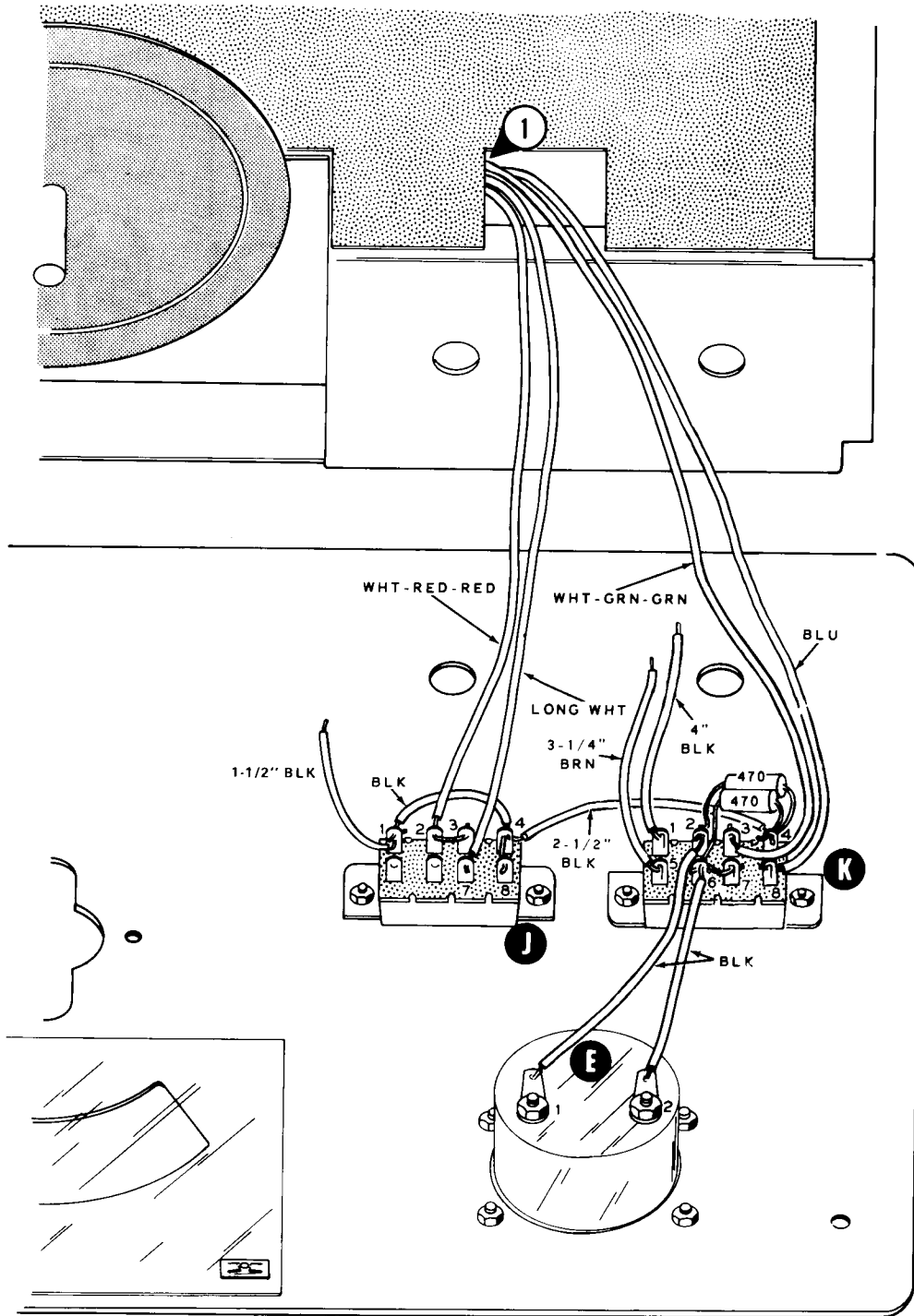
PICTORIAL 8-12
