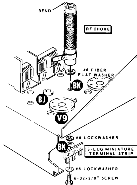
Detail 8-3C
