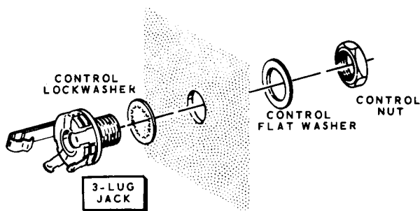
Detail 8-1C
