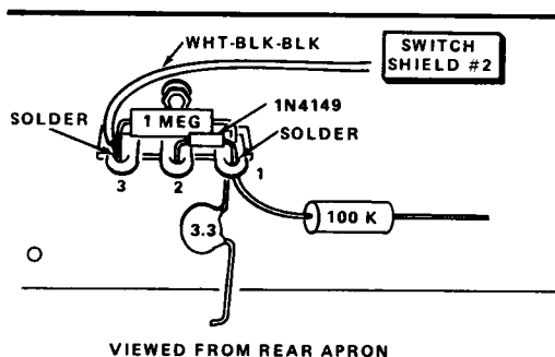
Detail 8-19D
