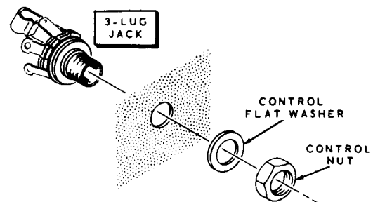
Detail 8-2M
