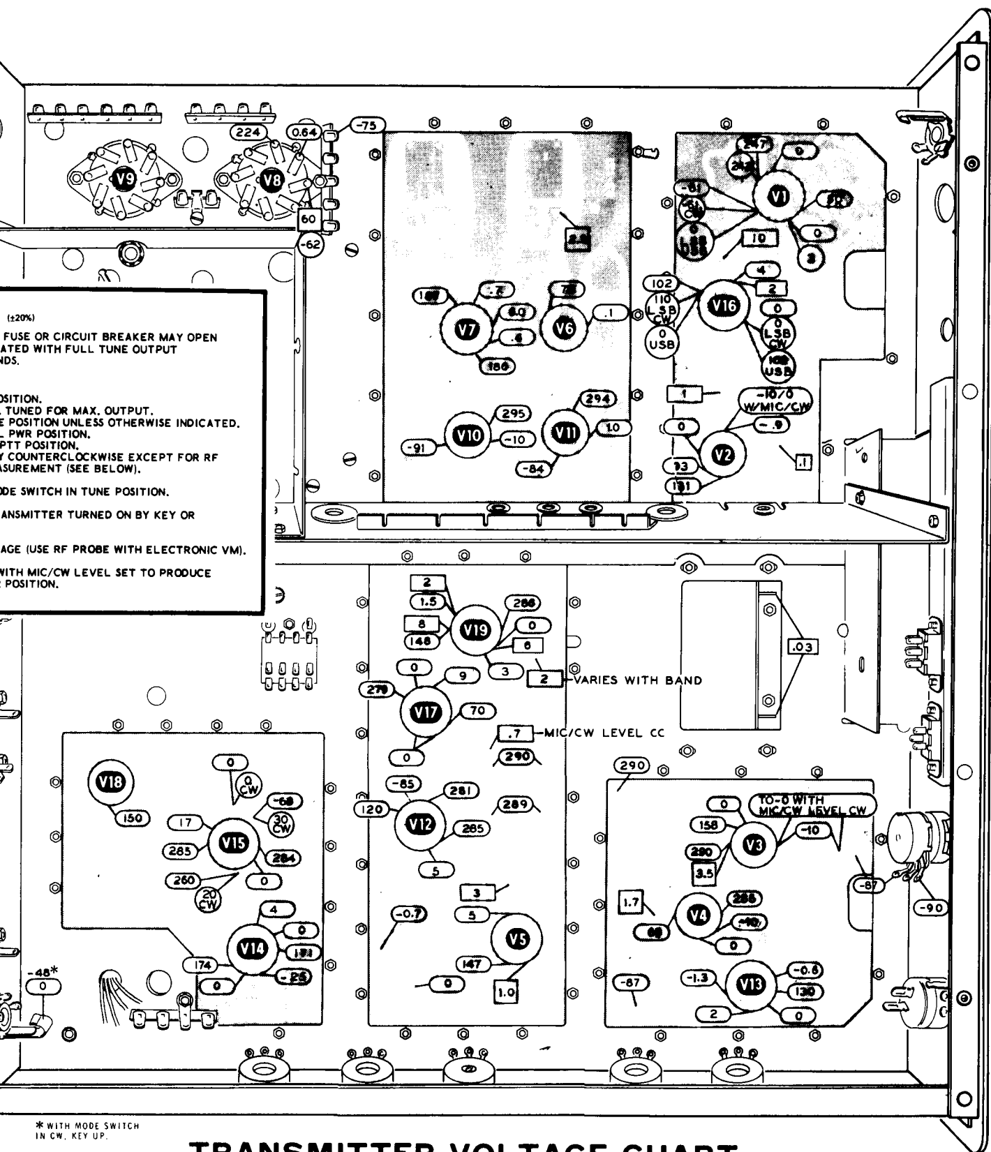
TRANSMITTER VOLTAGE CHART FIGURE 1-21
