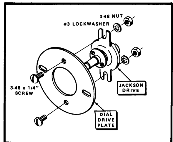
PICTORIAL 8-1
