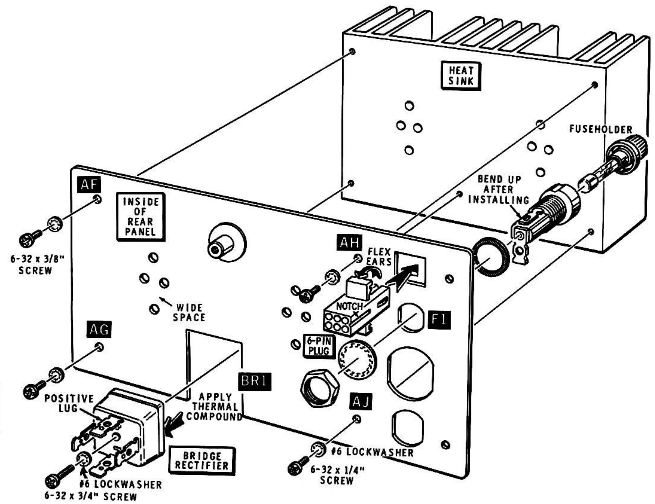
Detail 4-2A
