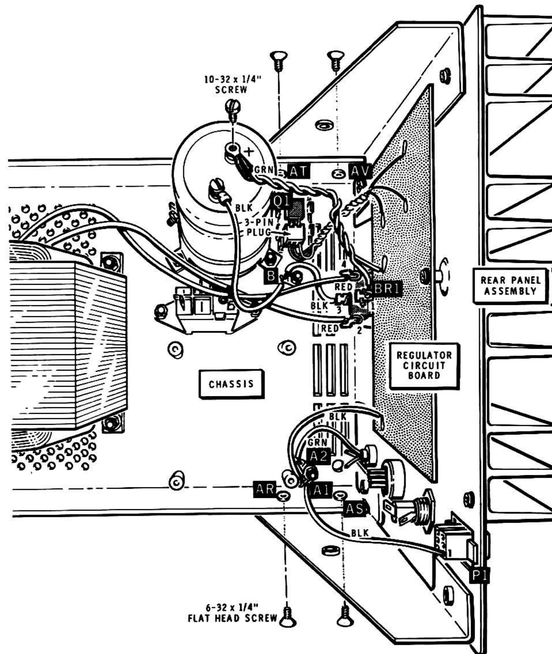
PICTORIAL 4-4
