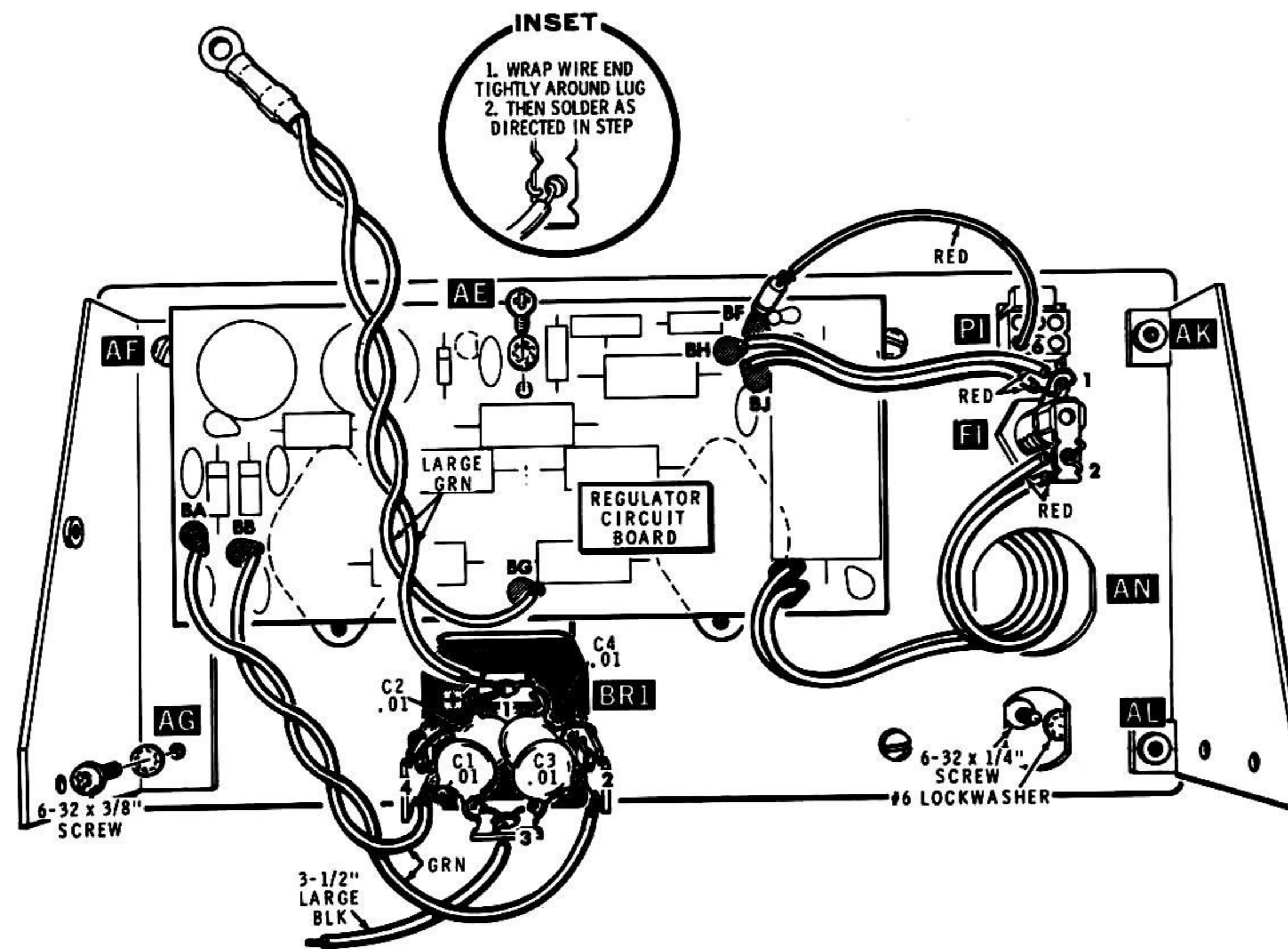
PICTORIAL 4-2
