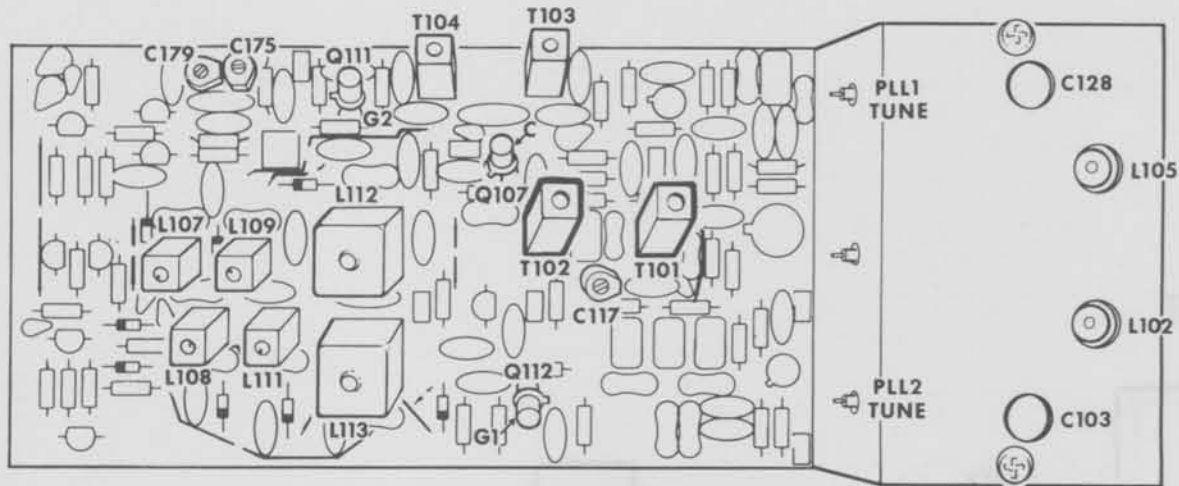
SYNTHESIZER CIRCUIT BOARD PICTORIAL 20-4
