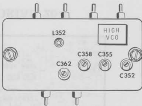
HIGH VCO ASSEMBLY PICTORIAL 20-6
