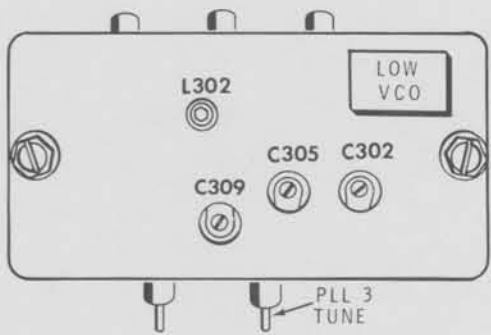
LO VCO ASSEMBLY PICTORIAL 20-5
