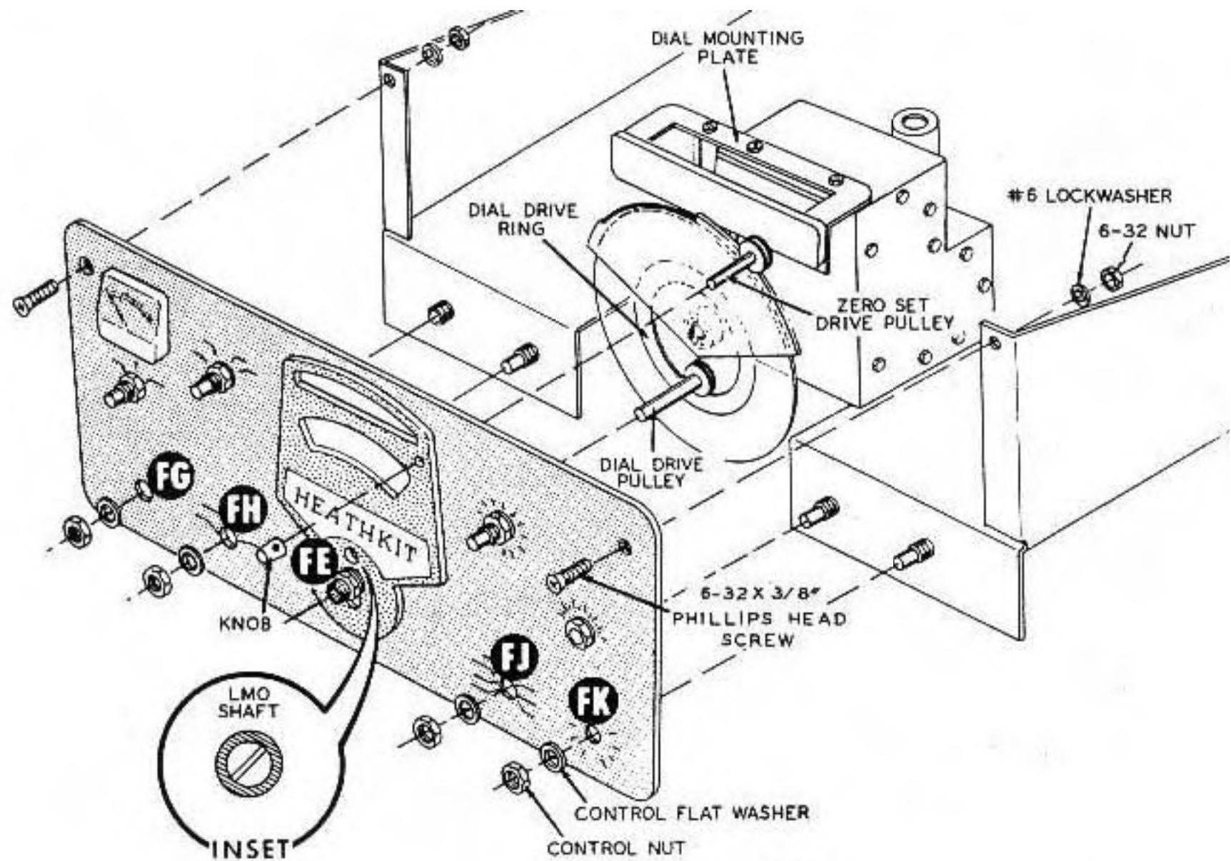
Detail 5-4B
