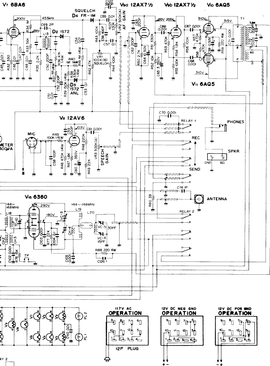
HA-1200 SCHEMATIC DIAGRAM
