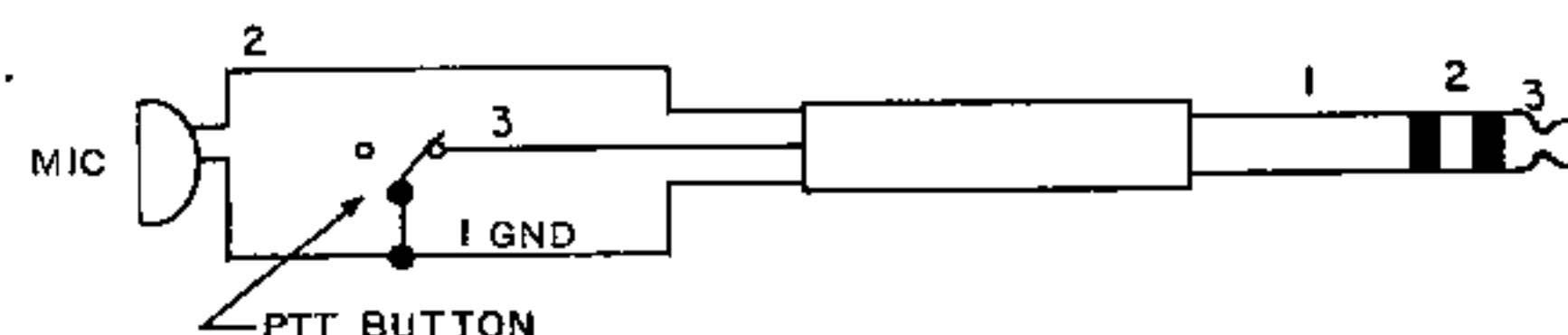
MICROPHONE CONNECTIONS
