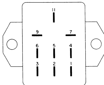
POWER CONNECTIONS
