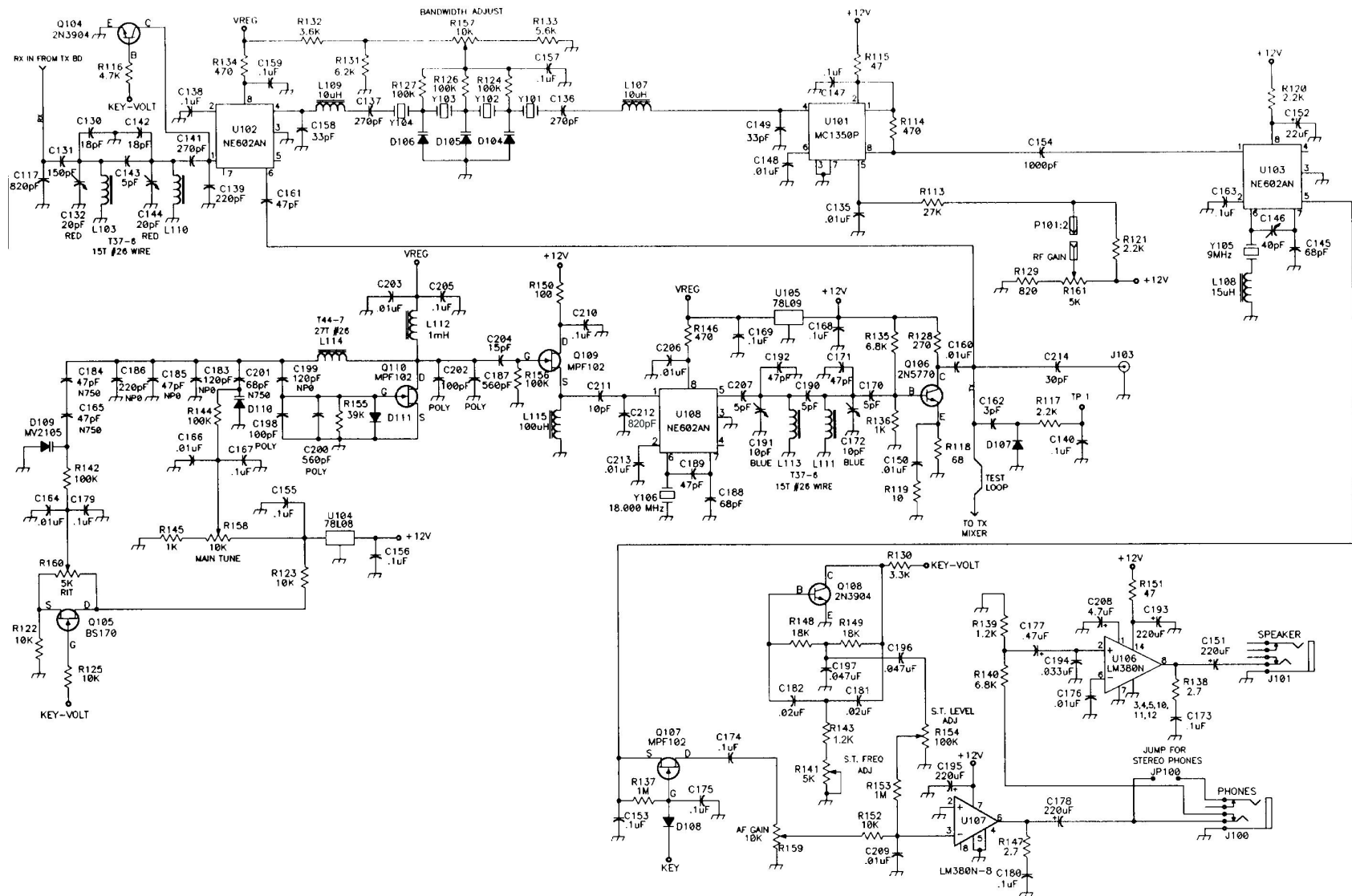
Receiver Section Schematic, 20M
