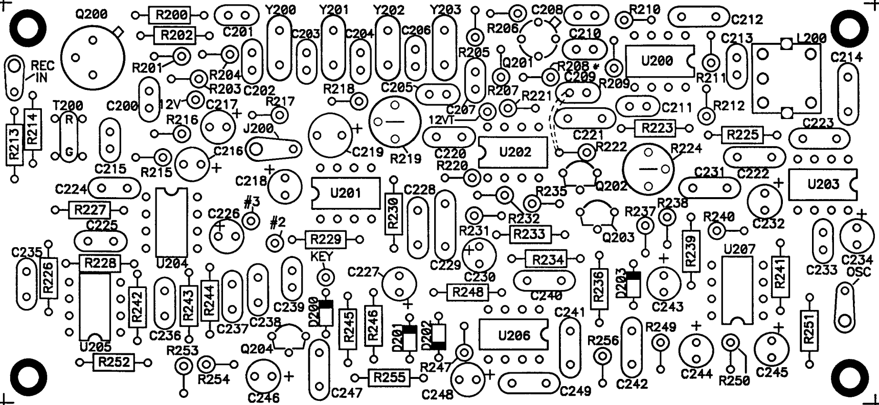
40-110 RECEIVER BOARD
