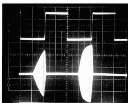
Figure 3—CW keying waveform for the PC-16000 with revised firmware installed to reduce the excessive delay. This shows the first two dits in full-break-in (QSK) mode using external keying at an equivalent keying speed of 60 WPM. The upper trace is the actual key closure; the lower trace is the RF envelope. Horizontal divisions are 10 ms. The transceiver was being operated at 100 W output at 14.2 MHz. Note some shortening of the first dit, which does not reach full output.
