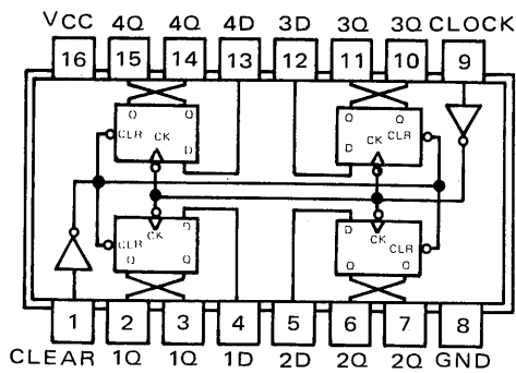
SN75491
