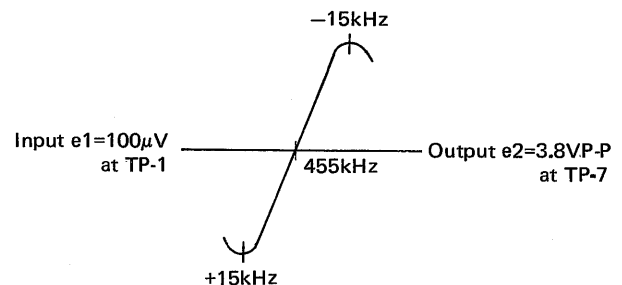
FIGURE 4. IF DISCRIMINATOR CURVE
