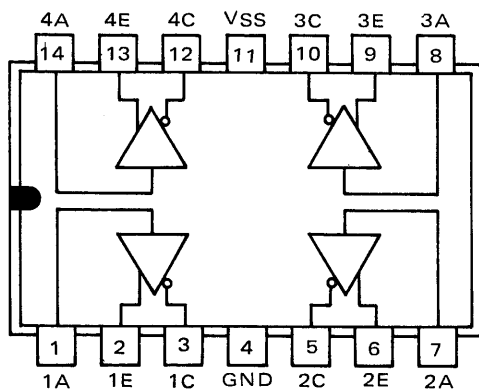
SN75491
