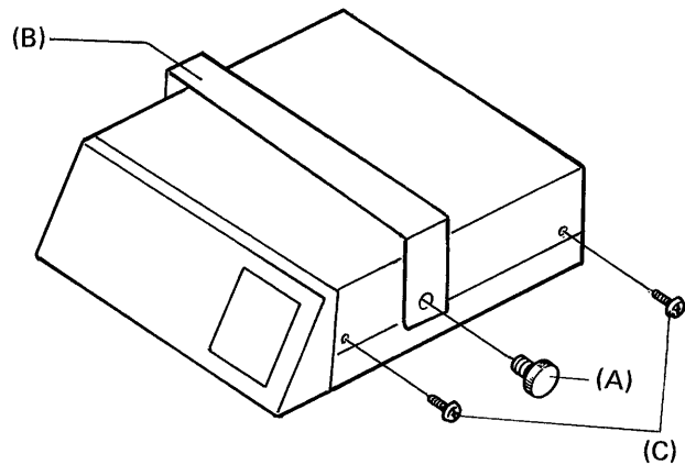
FIGURE 2. CHASSIS DISASSEMBLY
