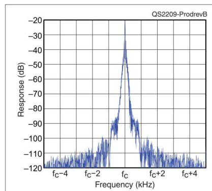
Figure B — The spectral display of the Elecraft K4D transmitter during keying sideband testing. Equivalent keying speed is 60 WPM using external keying and the default rise time setting. Spectrum analyzer resolution bandwidth is 10 Hz, and the sweep time is 30 seconds. The transmitter was being operated at 100 W PEP output on the 14 MHz band, and this plot shows the transmitter output \pm 5 kHz from the carrier. The reference level is 0 dBc, and the vertical scale is in dB.
