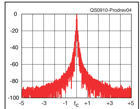
Figure 4 — Spectral display of the FLEX-3000 transmitter during keying sideband testing. Equivalent keying speed is 60 WPM using external keying. Spectrum analyzer resolution bandwidth is 10 Hz, and the sweep time is 30 seconds. The transmitter was being operated at 100 W PEP output on the 14 MHz band, and this plot shows the transmitter output \pm 5 kHz from the carrier. The reference level is 0 dBc, and the vertical scale is in dB.
