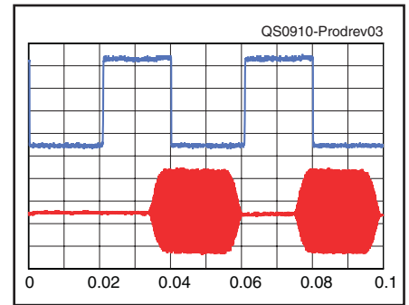
Figure 3 — CW keying waveform for the FLEX-3000 showing the first two dits in full-break-in (QSK) mode using external keying. Equivalent keying speed is 60 WPM. The upper trace is the actual key closure; the lower trace is the RF envelope. (Note that the first key closure starts at the left edge of the figure.) Horizontal divisions are 10 ms. The transceiver was being operated at 100 W output on the 14 MHz band.
