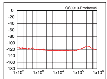
Figure 5 — Spectral display of the FLEX-3000 transmitter output during composite-noise testing. Power output is 100 W on the 14 MHz band. The carrier, off the left edge of the plot, is not shown. This plot shows composite transmitted noise 100 Hz to 1 MHz from the carrier. The reference level is 0 dBc, and the vertical scale is in dB.
