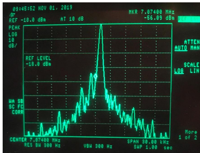
Transmitted 1-kHz USB tone.
