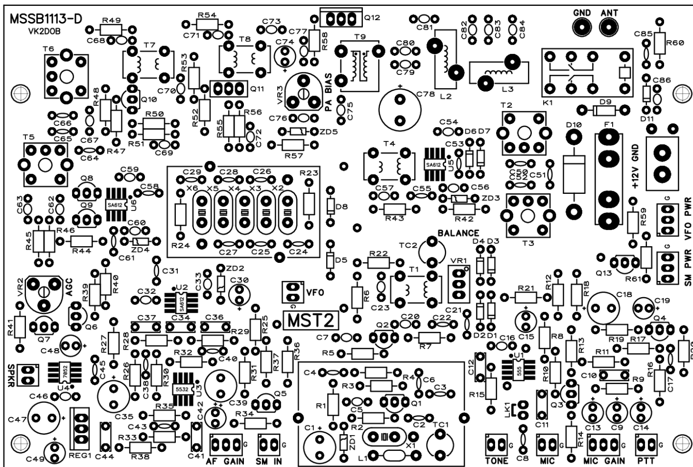
Figure 9 Component overlay
