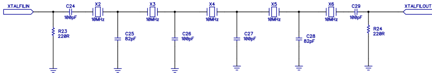
Crystal Filter
