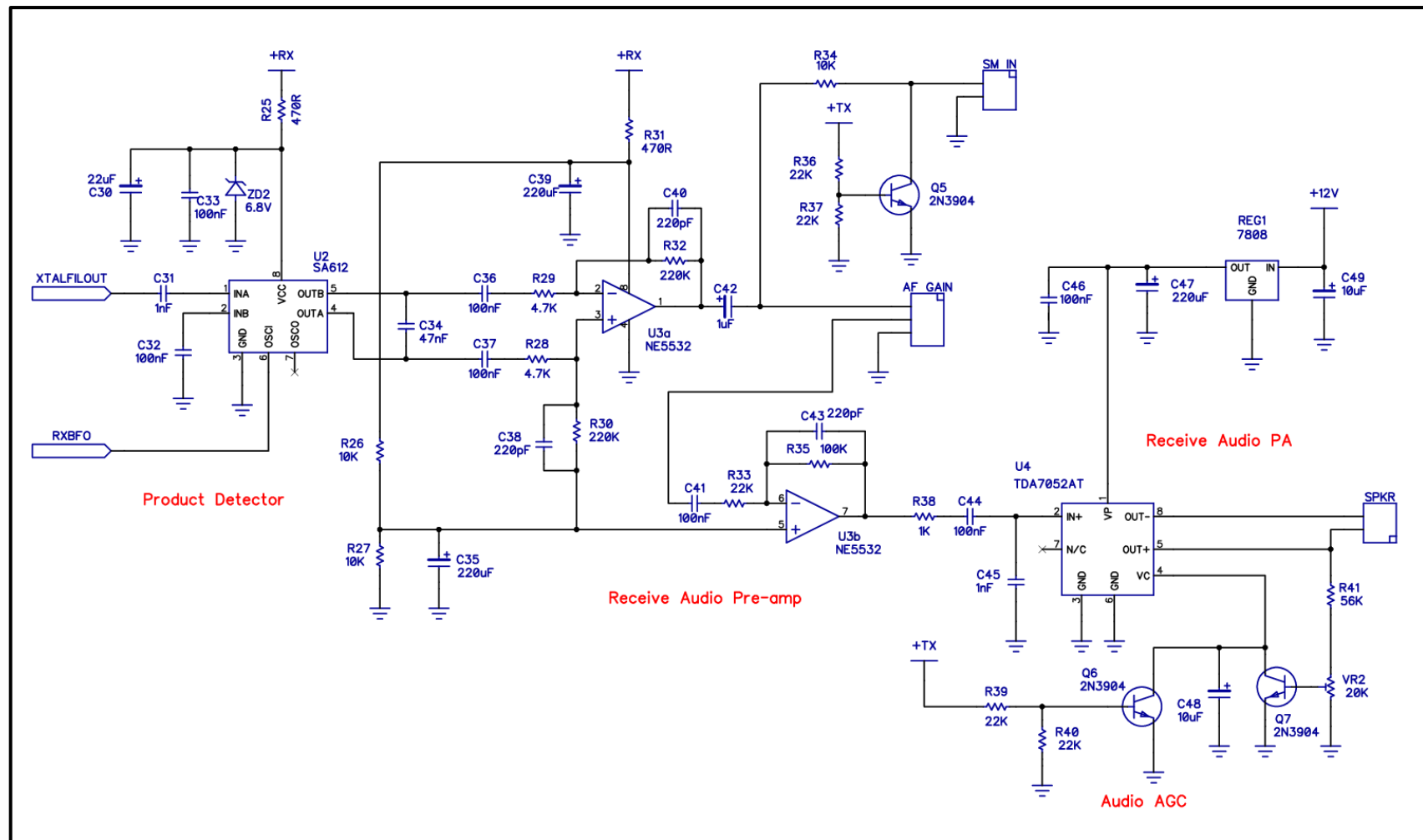
Figure 8 Receive audio
