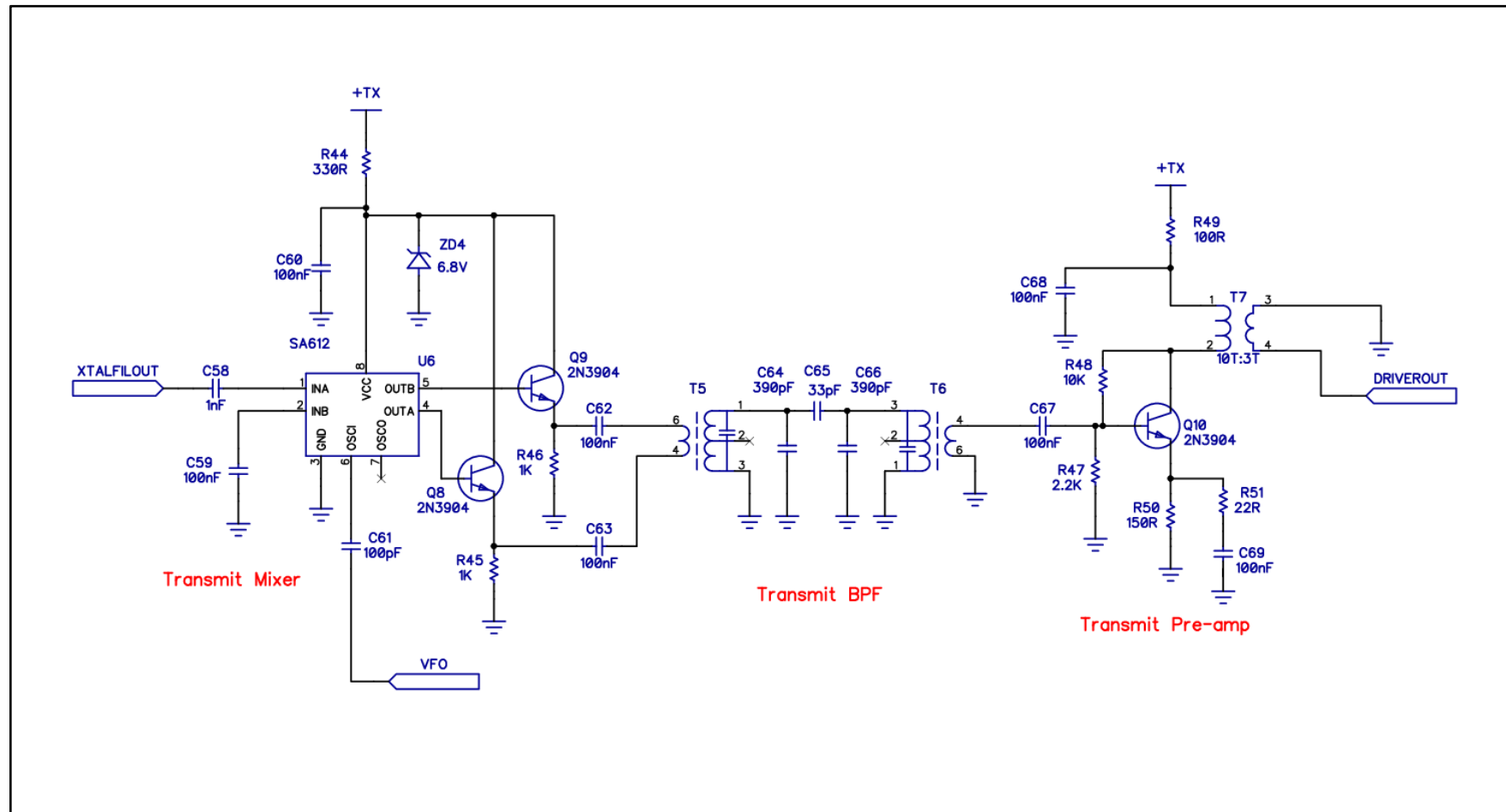
Figure 5 Transmit mixer
