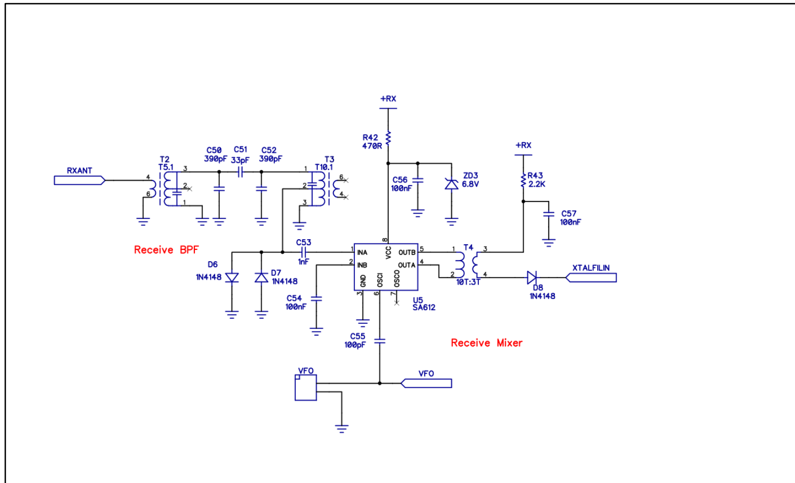
Figure 7 Receive mixer
