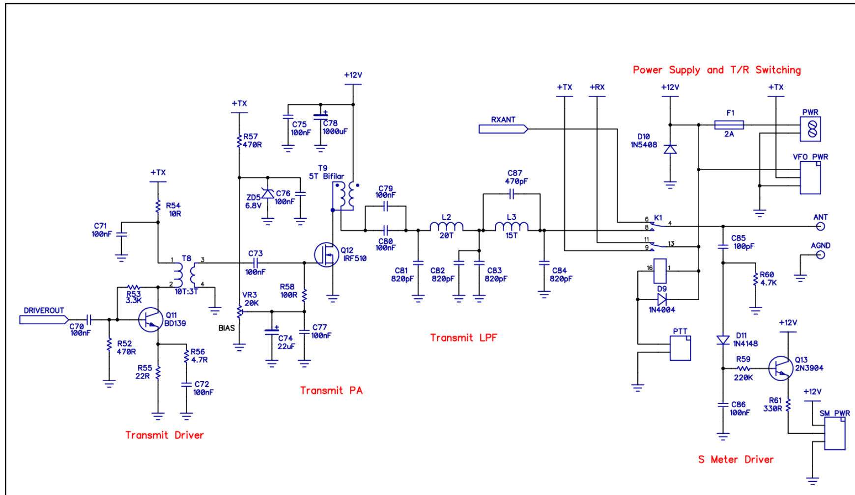
Figure 6 Power amplifier and RX/TX switching
