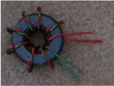
Figure 30. T3, 8T of 2 wire twisted pair wound on a FT37-43 Core
