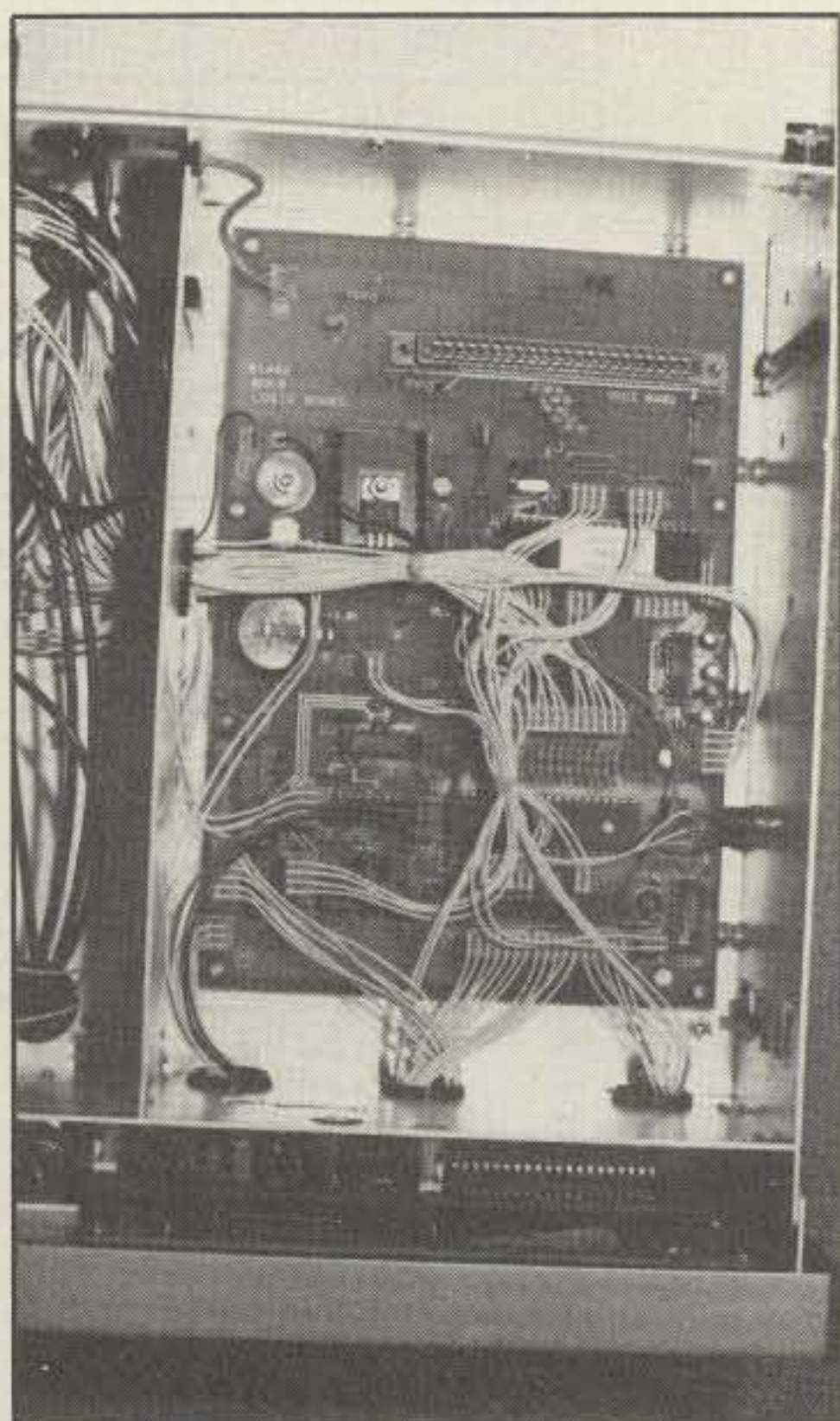
A closer look at the logic board. The round disc to the center left is the lithium memory back-up battery which will last about two years. It is easily user-replaceable. The connector to the top of the board is for an optional voice frequency readout board.
