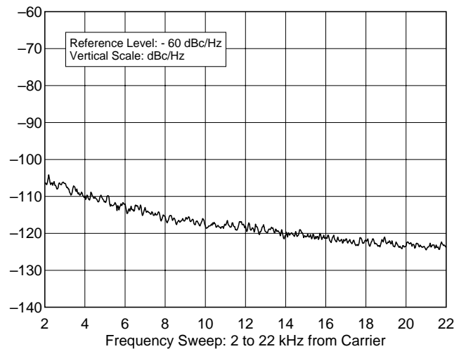
Yaesu FT-100 9D021081 432.020 MHz, Phase Noise, 100 W F:\SHARED\PROD_REV\TESTS\FT100.2ND\FT100P70.TXT
