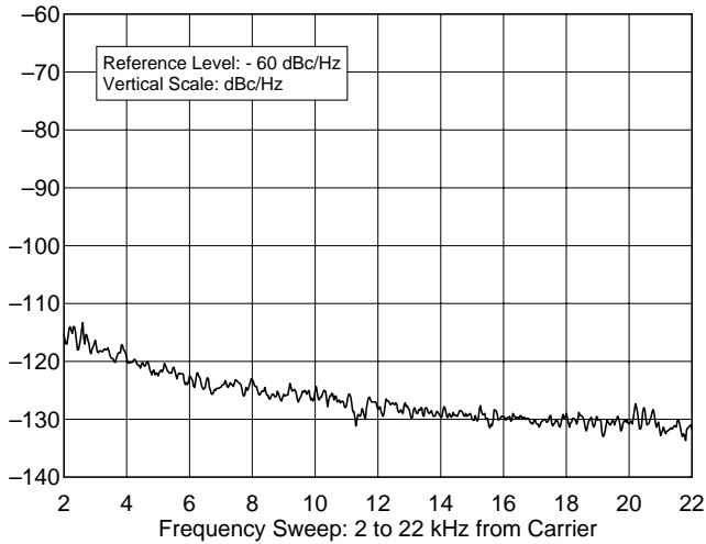
Yaesu FT-100 9D021081 14.020 MHz, Phase Noise, 100 W F:\SHARED\PROD_REV\TESTS\FT100.2ND\FT100P20.TXT
