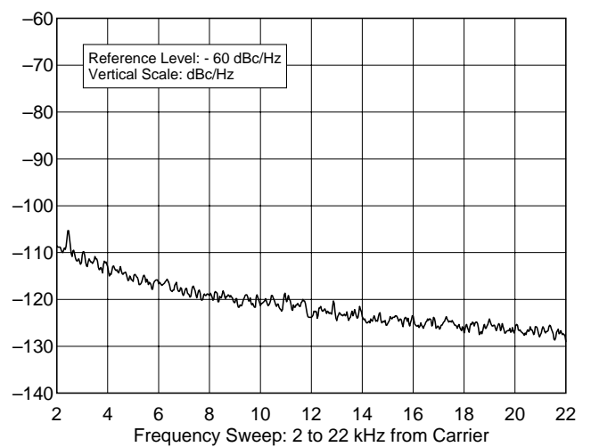
Yaesu FT-100 9D021081 144.020 MHz, Phase Noise, 100 W F:\SHARED\PROD_REV\TESTS\FT100.2ND\FT100P2M.TXT
