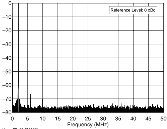
Yaesu FT-100 9D021081 1.9 MHz Band, Spectral Purity, 100 W F:\SHARED\PROD_REV\TESTS\FT100.2ND\FT100SLO.TXT
