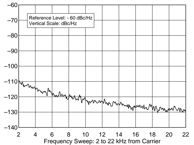
Yaesu FT-100 9D021081 50.020 MHz, Phase Noise, 100 W F:\SHARED\PROD_REV\TESTS\FT100.2ND\FT100P6M.TXT
