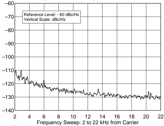
Yaesu FT-100 9D021081 3.520 MHz, Phase Noise, 100 W F:\SHARED\PROD_REV\TESTS\FT100.2ND\FT100P80.TXT
